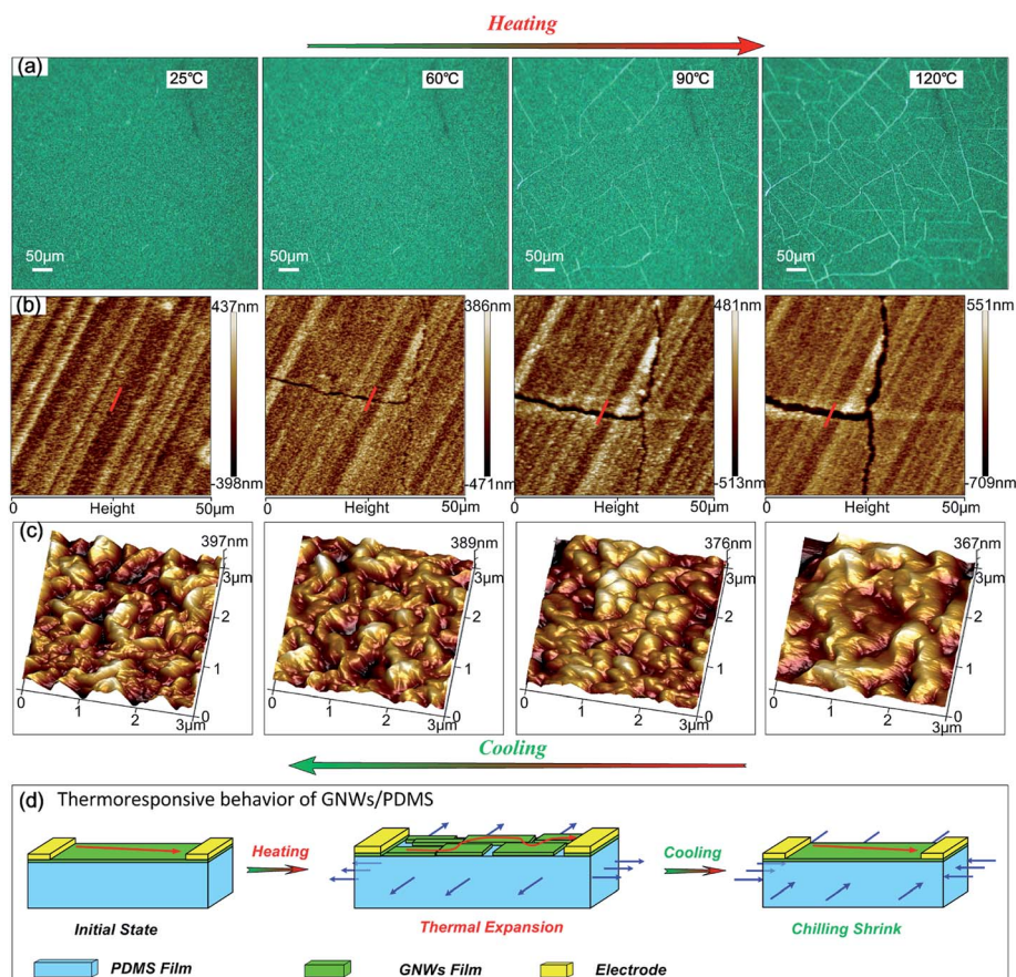
Fig. 4 Surface morphological change of GNWs film under different temperatures from 25 to 120^\circ\text{C} . (a) The optical microscopy image of GNWs film on PDMS ( 600 \times 600\text{ }\mu\text{m} ). (b) The AFM image of cracks evolution on GNWs film ( 50 \times 50\text{ }\mu\text{m} ). (c) The AFM cross-section of the crack region ( 3\text{ }\mu\text{m} ). (d) Schematic of thermal response/recovery of GNWs/PDMS film.
