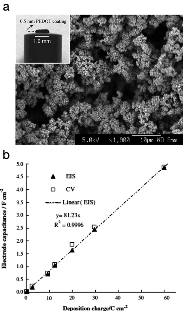
Fig. 18 (a) SEM micrograph of PEDOT electropolymerised via potentiostatic polymerisation (deposition charge: 30 C\text{ cm}^{-2} ). Inset: photograph of a PEDOT film ( 60 C\text{ cm}^{-2} ) on a Pt disc electrode. (b) Plot of the electrode specific capacitance as a function of polymerisation charge. Values measured by electrochemical impedance spectroscopy (EIS) and cyclic voltammetry (CV) are both presented. Reprinted from ref. 89 with permission from Elsevier.
