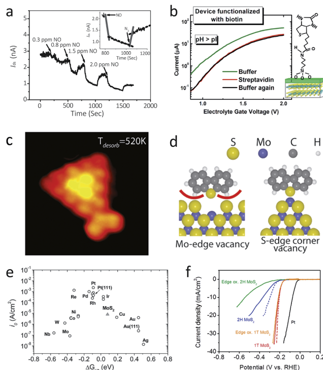
Fig. 8 (a) The current change of a double-layer \text{MoS}_2 transistor upon exposure of NO gas. The inset shows that the current level recovers upon purging with \text{N}_2 gas. 33 (b) Electron transport characteristics of \text{MoS}_2 -based biosensor with biotin decoration (left) and the schematic illustration of the device (right). 187 (c) and (d): A STM image of \text{MoS}_2 with thiophene adsorbed at the corner (c) and its molecular scheme showing the preference of S-edge corner vacancy for thiophene adsorption (d). 191 (e) A volcano plot of various metal electrodes for HER catalysis, including \text{MoS}_2 . 31 (f) Polarisation curve of \text{1T-MoS}_2 , \text{2H-MoS}_2 (before and after edge oxidation), and \text{Pt} electrode. 104 While edge oxidation significantly reduces the catalytic efficiency of \text{2H-MoS}_2 (blue to green), it does not affect \text{1T-MoS}_2 much (red to orange). Reproduced with permission from: (a) ref. 33 © 2012 John Wiley and Sons; (b) ref. 187 © 2014 American Chemical Society; (c) and (d) ref. 191 © 2010 American Chemical Society; (e) ref. 31 © 2007 American Association for the Advancement of Science; (f) ref. 104 © 2013 American Chemical Society.
