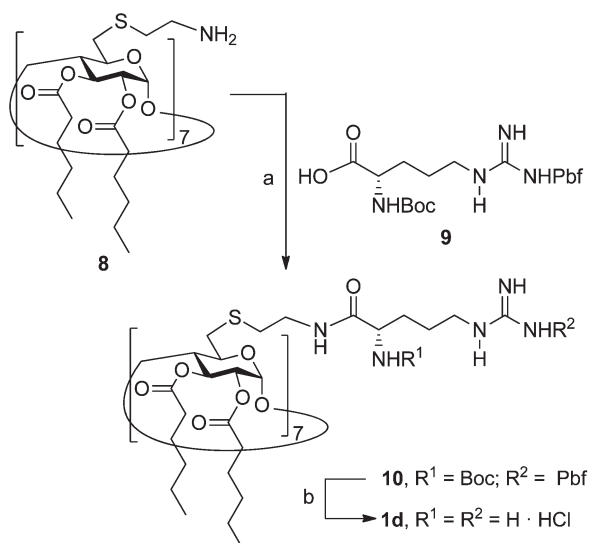
Scheme 2 Synthesis of amide-linked polyarginine βCD derivative 1d . Reagents and conditions: (a) HBTU, DIPEA, DCM, rt, 12 h, 68%; (b) (i) 95 : 2.5 : 2.5 TFA–TIS–DCM, rt, 1 h; (ii) 0.1 M HCl, quantitative. Pbf: 2,2,4,6,7-pentamethyl-dihydrobenzofuran-5-sulfonyl. HBTU: o -(benzotriazol-1-yl)- N,N,N',N' -tetramethyluronium hexafluorophosphate. DIPEA: Diisopropyl ethyl amine. TIS: triisopropylsilane.
