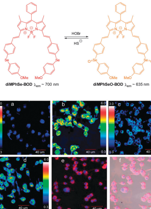
Fig. 110 Confocal fluorescence images of the redox cycles between HOBr and \text{H}_2\text{S} in RAW264.7 cells. Macrophage cells. (a) Control; (b) diMPhSe-BOD -loaded cells with \text{H}_2\text{O}_2 , EPO, and KBr; (c) cells in (b) after addition of \text{HS}^- ; (d) (c) was treated with a second dose of \text{H}_2\text{O}_2 , EPO and KBr; (e) overlay of images showing fluorescence from diMPhSe-BOD and Hoechst dye; (f) overlay of bright-field, diMPhSe-BOD , and Hoechst dye images. Image reproduced with permission. 335
