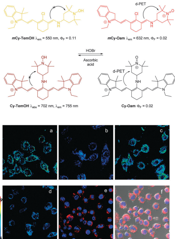
Fig. 109 Top: structure of mCy-TemOH and Cy-TemOH and their reaction with \text{BrO}^- . Bottom: ratiometric fluorescence images ( F_{632}/F_{550} ) of living RAW264.7 cells with mCy-TemOH (a)–(d). Pseudo color images represent the ratio of emission intensities. (a) Control. (b) mCy-TemOH -loaded cells incubated with \text{H}_2\text{O}_2 , EPO and KBr. (c) mCy-TemOH loaded, EPO, and \text{H}_2\text{O}_2 treated cells incubated with glutathione S-transferase, then ascorbic acid. (d) Cells exposed to a second dose of EPO, KBr and \text{H}_2\text{O}_2 . (e) and (f) Confocal microscopy imaging for subcellular locations of mCy-TemOH in living RAW264.7 cells. (e) Cells incubated with mCy-TemOH (red) and co-staining with Hoechst dye (blue). (f) Overlay of (e) and its bright-field image. Image reproduced with permission. 334
