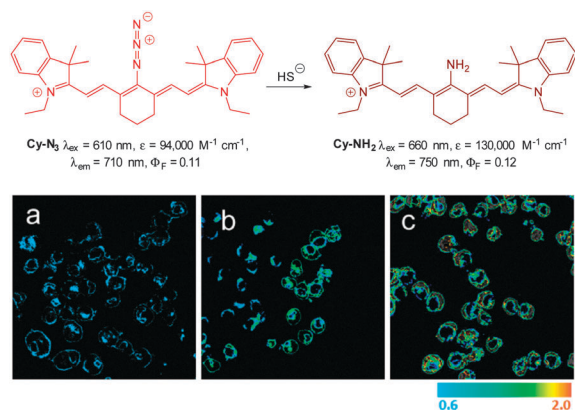
Fig. 56 Top: structure and reaction of Cy-N 3 with HS − . Bottom: ratio-metric fluorescence images (F 750 /F 710 ) of living RAW264.7 macrophage cells with Cy-N 3 . Images displayed in pseudo colour represent the ratio of emission intensities. (a) Cells were pretreated with PMA before loading Cy-N 3 . (b) Cells incubated with Cy-N 3 . (c) RAW264.7 cells incubated with NaSH and Cy-N 3 was added. Image reproduced with permission. 227
