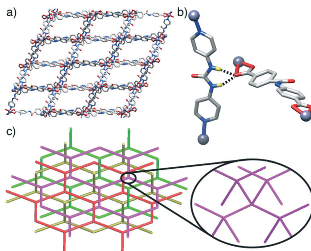
Fig. 4 a) Crystal packing in the solid-state structure of [\text{Zn}(\text{L2})(\text{P3})]_n viewed down the crystallographic a axis to show one-dimensional pores. b) A bifurcated hydrogen bonding interaction in the crystal structure, between the urea unit of P3 and a carboxylic oxygen atom of a molecule of L2 from an adjacent net. c) The four-fold interpenetrated dia topology, with inset, adopted by both [\text{Zn}(\text{L1})(\text{P3})]_n and [\text{Zn}(\text{L2})(\text{P3})]_n .
