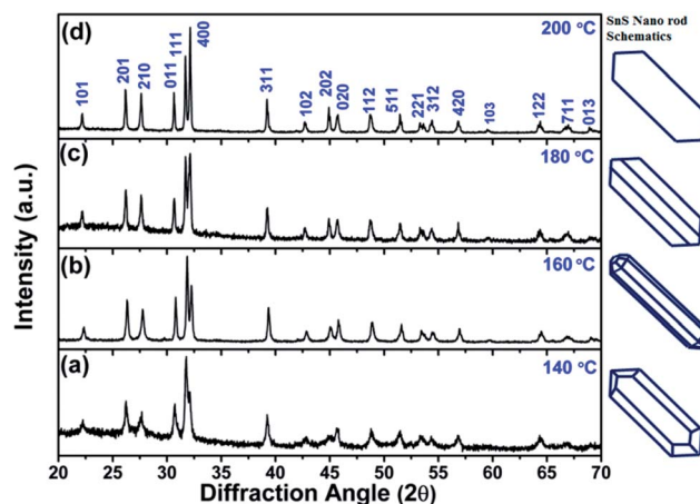
Fig. 5 Powder X-ray diffraction patterns of SnS nanorods synthesized at (a) 140 °C, (b) 160 °C, (c) 180 °C and (d) 200 °C.
