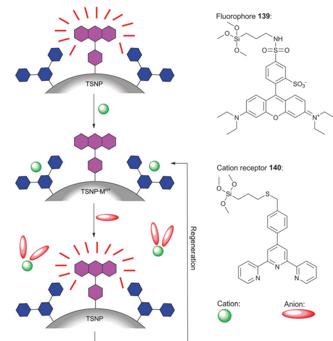
Scheme 17 Design concept of the anion quencher displacement assay (QDA) involving terpyridine-sulforhodamine functionalised nanoparticle (TSNP) and a metal ion quencher, along with the structure of fluorescent dye 139 (magenta) and cation receptor 140 (blue).
