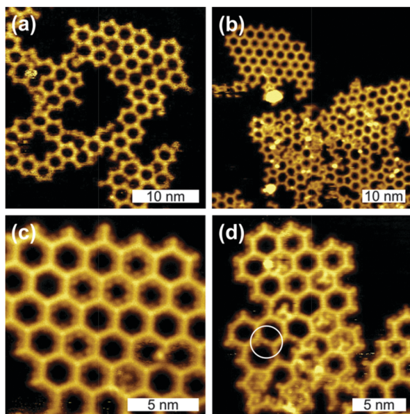
Fig. 3 STM images of covalent networks on Ag(111). BIB was deposited at RT ((a) -1.9 V, 24.7 pA) or deposited onto a preheated sample at 150 °C (b) – (d). Subsequently, both samples were tempered up to 250 °C ((b) + (c) 4.6 pA, +3.9 V, (d) 5.5 pA, +2.6 V). The circle in (d) marks a still present organometallic bond in a disordered domain.
