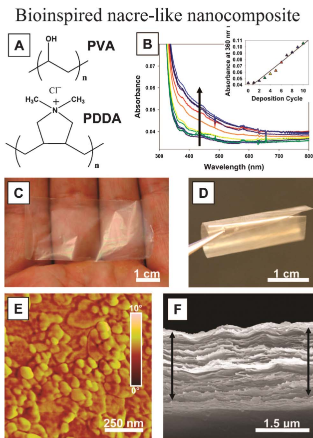
Fig. 19 (a) Structure of PVA and PDDA polymers; (b) UV-vis spectra for the first 10 bilayers of deposition (arrow indicates increasing absorbance, inset represents absorbance at 360 nm as a function of the bilayer); (c, d) optical images of a free-standing film of (PVA-MTM) 300 showing very high transparency and flexibility; (e) AFM phase image of a single PVA-MTM bilayer; (f) SEM image of the cross section of a 300-bilayer PVA-MTM composite showing its laminar architecture. The films in SEM can be slightly expanded due to separation of the layers resulting from the shearing force of the razor blade used for cutting the test samples. 60
