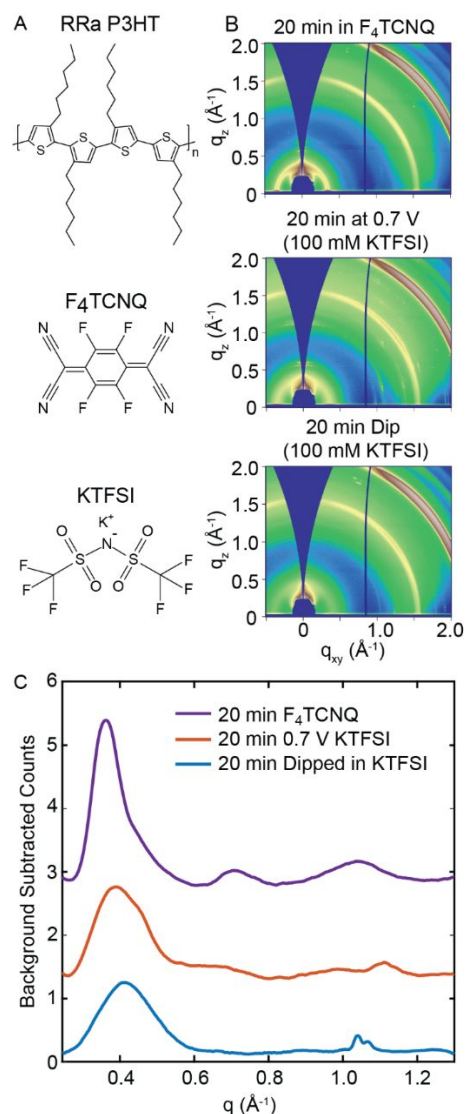
Figure 1. 2D GIWAXS diffractograms and radially integrated diffractograms of RRa P3HT under different conditions. (A) Chemical structures of RRa P3HT, F 4 TCNQ, and KTFSI. (B) GIWAXS diffractograms of a RRa P3HT thin film immersed in 10 mg/mL F 4 TCNQ for 20 min (top), doped at 0.7 V vs Ag/AgCl for 20 min (middle), and immersed in an aqueous 100 mM KTFSI electrolyte for 20 min (bottom). (C) Radially integrated and background subtracted GIWAXS diffractograms of the RRa P3HT thin films.
