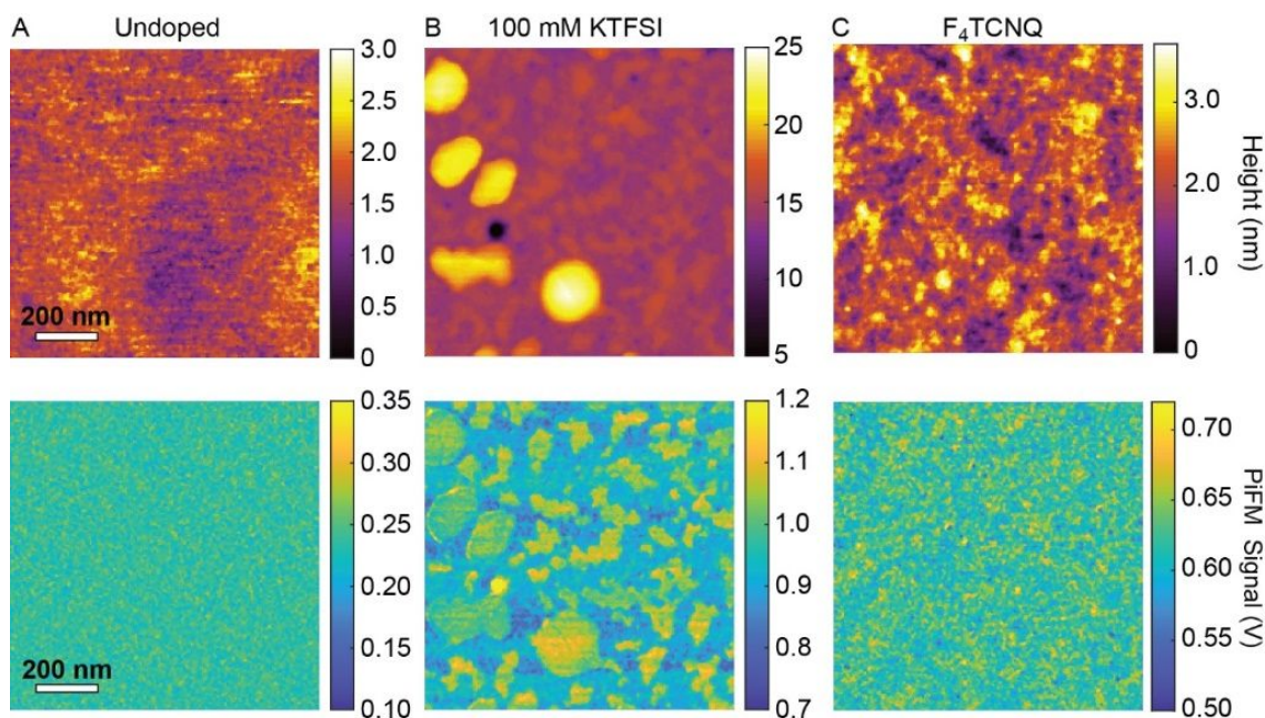
Figure 2. PiFM images of RRa P3HT films that underwent electrochemical and chemical doping. AFM topography and PiFM nanoscale infrared images of (A) an undoped RRa P3HT film, (B) a RRa P3HT thin film doped for 20 min in an aqueous 100 mM KTFSI electrolyte, and (C) a RRa P3HT film doped in a F 4 TCNQ solution for 20 min.
