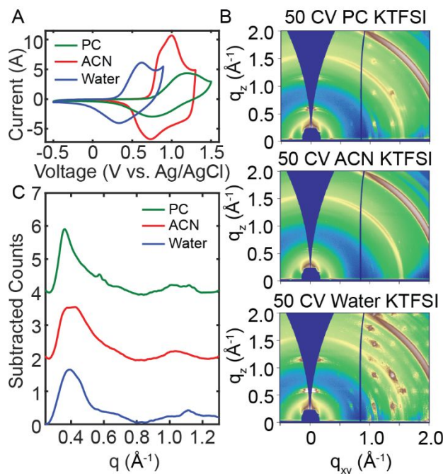
Figure 5. Comparison between using different electrolyte solvents. (A) CVs of RRa P3HT thin films in water, acetonitrile, and propylene carbonate (100 mM KTFSI). (B) GIWAXS diffractograms of P3HT thin films after undergoing 50 CVs in water (bottom), acetonitrile (middle) and propylene carbonate (top) (100 mM KTFSI). (C) ITO background subtracted linecuts of each thin film after undergoing 50 CVs.
