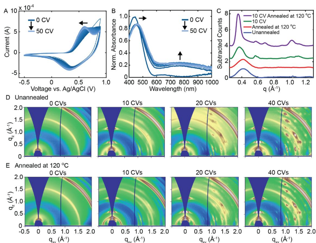
Figure 3. Impact of performing a series of CVs on the structure of RRa P3HT thin films. (A) A series of 50 CVs acquired of RRa P3HT from -0.5 to 0.9 V at a scan rate of 0.1 V/s. (B) UV/Vis spectra collected every 5 CVs after a 45 s dedoping step at -0.5 V vs. Ag/AgCl. (C) Background subtracted radially integrated GIWAXS diffractograms of four RRa P3HT thin films: not annealed, annealed at 120 °C for 20 min, after performing 10 CVs in aqueous 100 mM KTFSI, and after performing 10 CVs followed by a 20 minute 120 °C annealing step. (D) A series of 2D GIWAXS diffractograms of RRa P3HT after 0, 10, 20, and 40 CVs. (E) A series of 2D GIWAXS diffractograms of RRa P3HT after 0, 10, 20, and 40 CVs followed by thermal annealing at 120 °C for 20 min.
