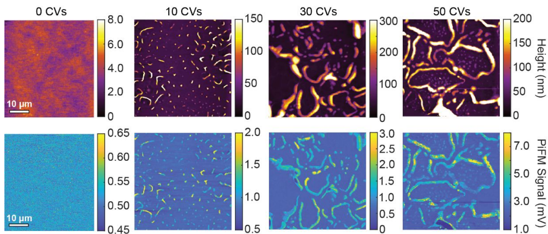
Figure 4. AFM topography and PiFM images of a RRa P3HT thin film upon increasing numbers of CVs performed in aqueous 100 mM KTFSI after a 40 s -0.5 V (vs. Ag/AgCl) dedoping step. 50 x 50 μm AFM topography and PiFM images are collected of an undoped RRa P3HT thin film, as well as RRa P3HT thin films that underwent 0, 10, 30, and 50 CVs.
