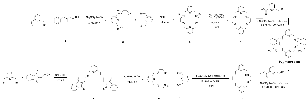
Scheme 1. Previously reported synthetic approach of dipyrindine macrocyclic backbone (top) and improved synthetic approach of dipyrindine macrocyclic backbone by using metal ion template synthesis (bottom).
