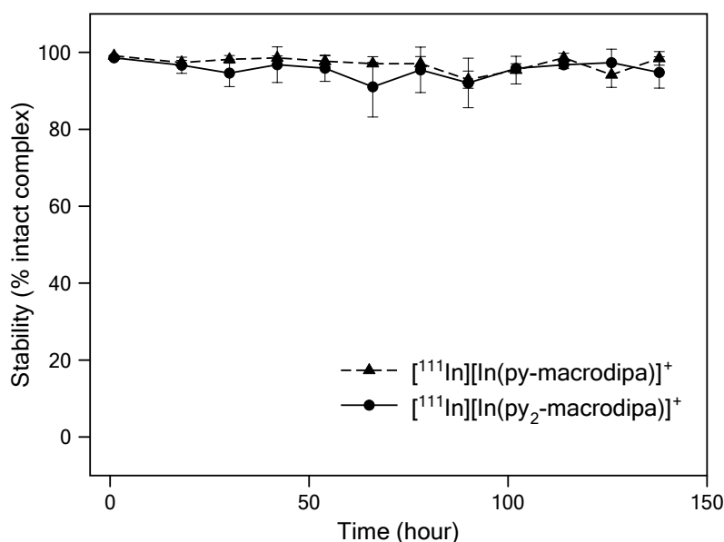
Figure 5. Stability of [ 111 In][In(py-macrodipa)] + and [ 111 In][In(py 2 -marodipa)] + in human serum at 37 °C.
