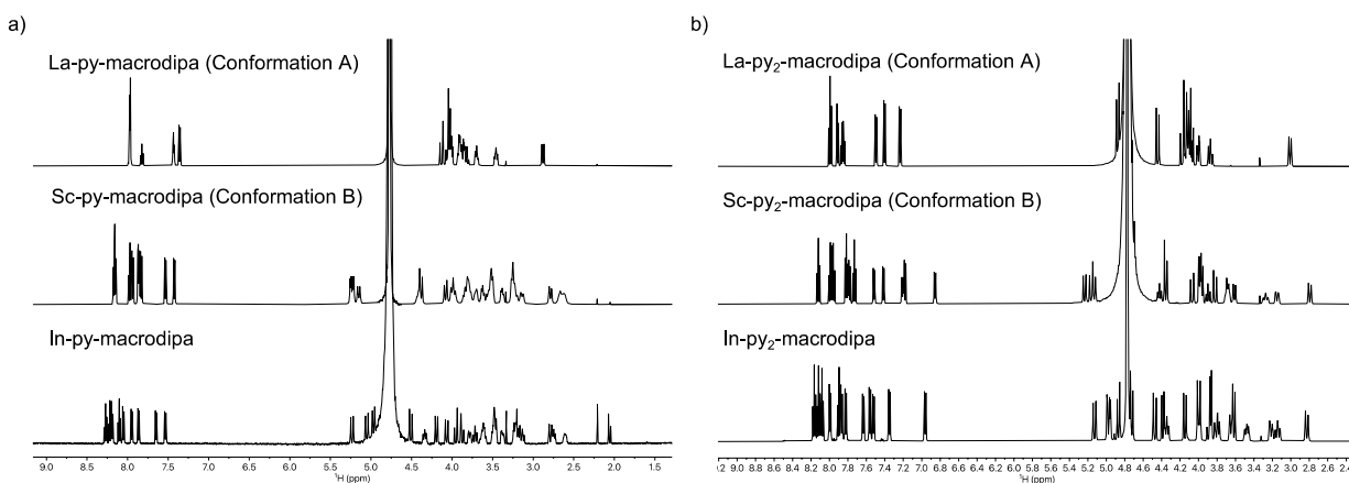
Figure 1. a) ^1\text{H} NMR spectra of [\text{La}(\text{py-macrodipa})]^+ , [\text{Sc}(\text{py-macrodipa})]^+ and [\text{In}(\text{py-macrodipa})]^+ (500 MHz, \text{D}_2\text{O} , pD 5, 25 °C). b) ^1\text{H} NMR spectra of [\text{La}(\text{py}_2\text{-macrodipa})]^+ , [\text{Sc}(\text{py}_2\text{-macrodipa})]^+ , and [\text{In}(\text{py}_2\text{-macrodipa})]^+ (500 MHz, \text{D}_2\text{O} , pD 5, 25 °C).
