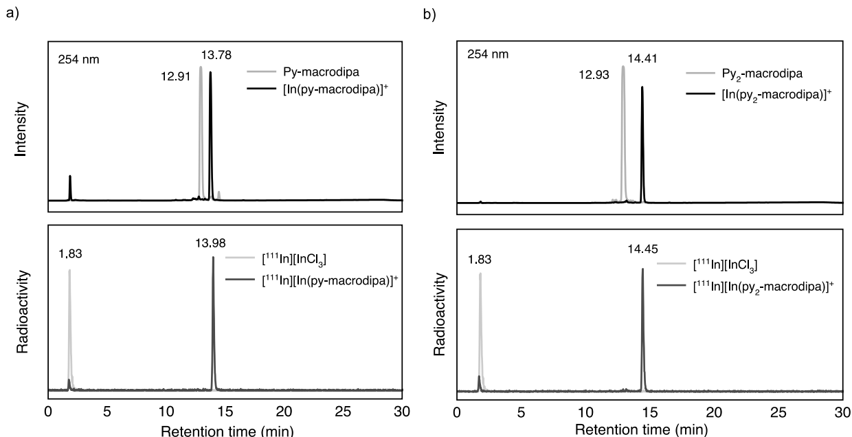
Figure 5. a) UV-vis-HPLC chromatogram (254 nm) of nonradioactive [In(py-macrodipa)] + and py-macrodipa (top) compared with radio-HPLC chromatogram of [ 111 In][In(py-macrodipa)] + and [ 111 In]InCl 3 (bottom). b) UV-vis-HPLC chromatogram (254 nm) of nonradioactive [In(py 2 -macrodipa)] + and py 2 -macrodipa (top) compared with the radio-HPLC chromatogram of [ 111 In][In(py 2 -macrodipa)] + and [ 111 In]InCl 3 (bottom).
