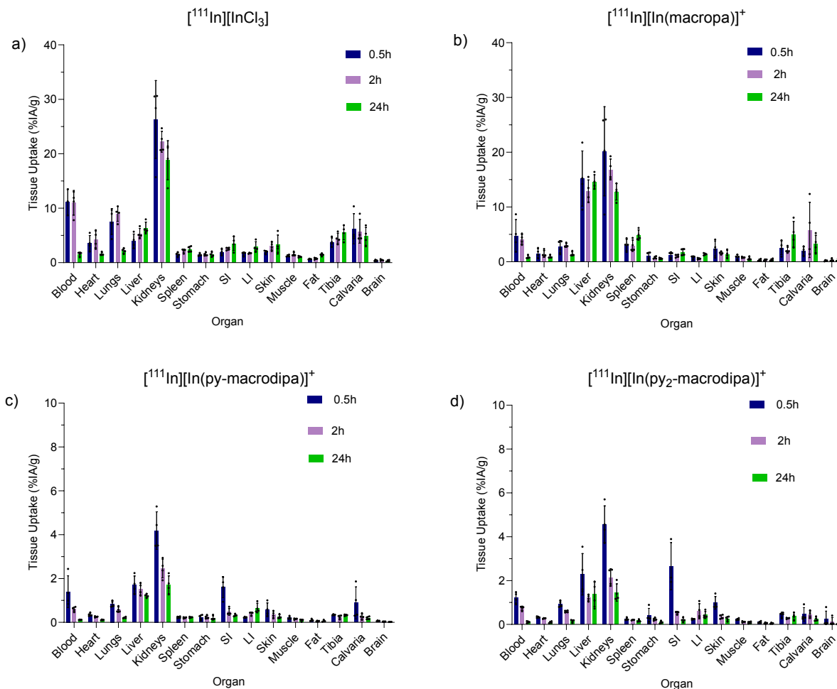
Figure 6. In vivo biodistribution of [^{111}\text{In}]\text{InCl}_3 , [^{111}\text{In}][\text{In}(\text{macropa})]^+ , [^{111}\text{In}][\text{In}(\text{py-macrodipa})]^+ , and [^{111}\text{In}][\text{In}(\text{py}_2\text{-macrodipa})]^+ following retro-orbital injection in mice. Four Naive Swiss Webster females of 4–6 weeks old were sacrificed after 0.5, 2, and 24 h. Values for each time point are given as percent injected activity per gram tissue (%IA/g).
