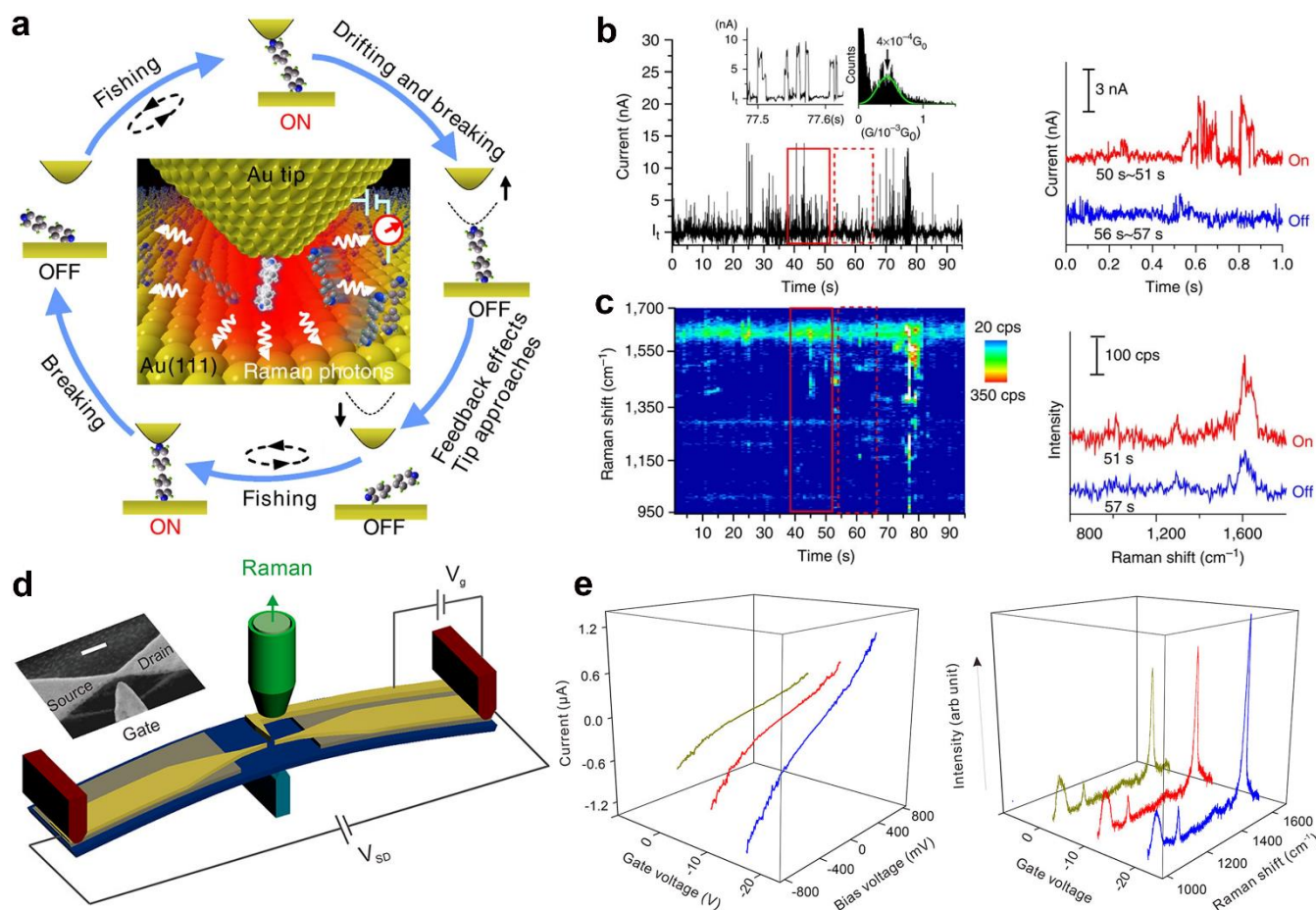
Fig. 11 (a) A schematic illustration of the 'fishing-mode' TERS. (b-c) Simultaneous conductance and TERS measurement of 4bipy by 'fishing-mode' TERS. Upper: Conductance versus time; Lower: TERS spectra versus time. Figures reproduced with permission from ref. 45. Copyright 2011, Springer Nature. (d) Experimental schematic of side-gating Raman scattering. Scale bar is 100 nm for the inset SEM image of the MCBJ chip with a side-gate electrode. (e) SERS spectra recorded at different gate voltages (left panel) and I - V curves of 1,4-benzenedithiol MJ upon different gate voltages (right panel). Figures reproduced with permission from ref. 124. Copyright 2018, American Chemical Society.
