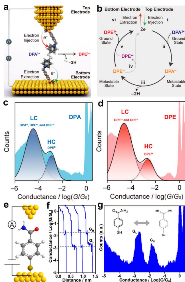
Fig. 3 (a) Schematic representation of electron-catalyzed DPA 2+ to DPE 2+ dehydrogenation at an STM junction. (b) A plausible mechanism for the electron catalyzed DPA 2+ -to-DPE 2+ dehydrogenation. (c and d) 1D conductance-displacement histograms of DPA 2+ -to-DPE 2+ , respectively. Figures reproduced with permission from ref. 57. Copyright 2021, American Chemical Society. (e) Schematic illustration of the STMBJ measurement of an SMJ containing an MBAm molecule. (f) Typical conductance decay traces were recorded in STMBJ measurements at 0.1 V bias in DI water. (g) Logarithm-binned conductance histogram for MBAm, showing two distinct conductance peaks at 10 -2.72 and 10 -1.78 G 0 , respectively. Figures reproduced with permission from ref. 58. Copyright 2021, American Chemical Society.
