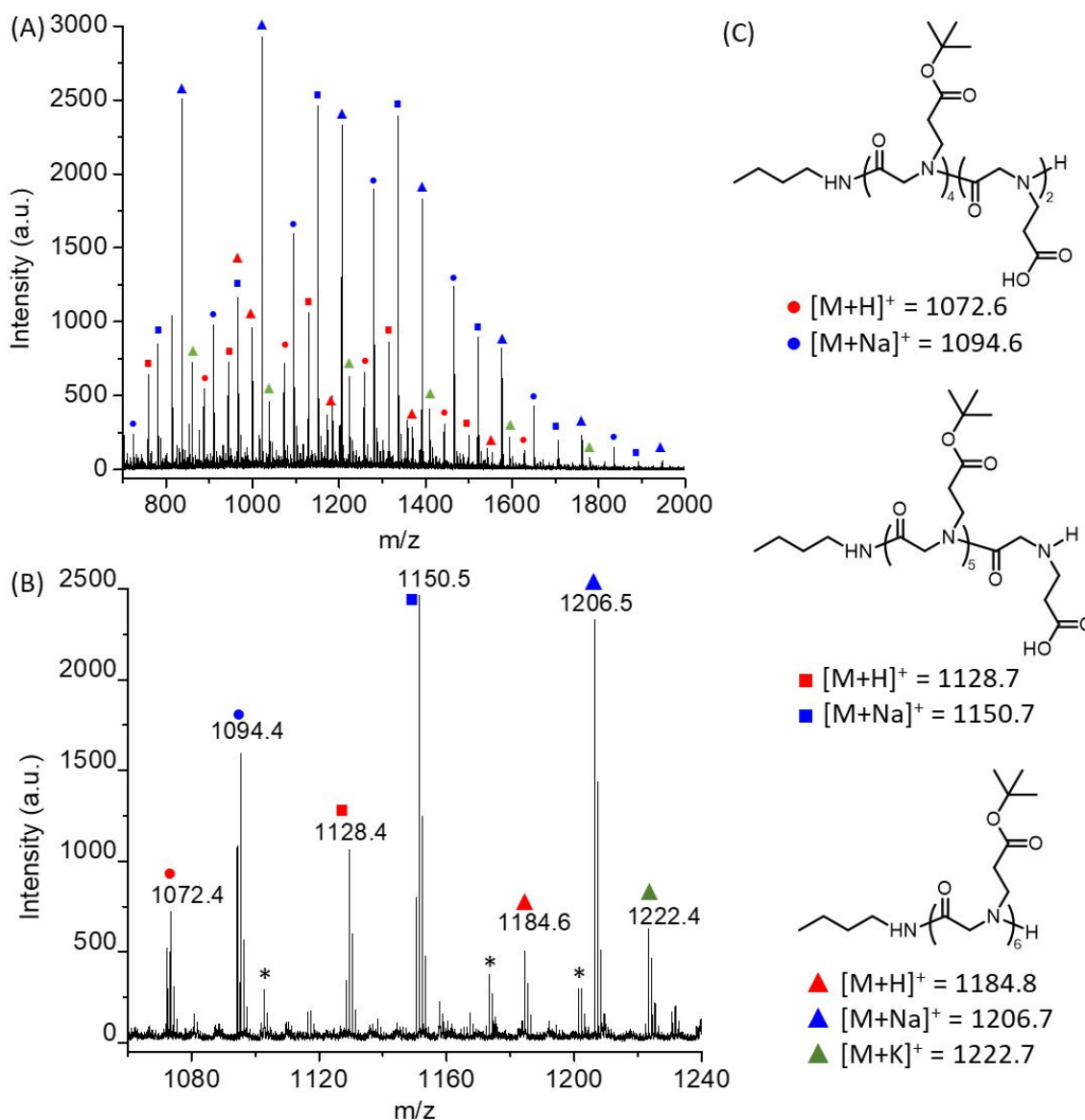
Figure 2. (A) Full and (B) expanded MALDI-TOF MS spectrum of a low molecular weight poly( N -(3- tert -butoxy-3-oxopropyl) glycine) obtained from the butylamine-initiated ROPs of ^t\text{BuO}_2\text{Pr-NCA} in toluene together with (C) the structural assignment of the molecular ions and corresponding calculated m/z values. * ( m/z = 1101.7, 1173.4 and 1201.4 ) correspond to poly( N -(3- tert -butoxy-3-oxopropyl) glycine) species whose end-group structures are presently unclear.
