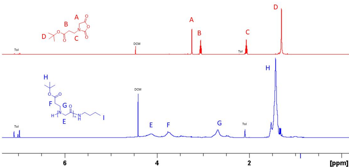
Figure 1. (A) ^1\text{H} NMR spectra of ^t\text{BuO}_2\text{Pr-NCA} and (B) poly( N -(3- tert -butoxy-3-oxopropyl) glycine) in toluene- d_8 that were obtained by the butylamine-initiated ROPs of ^t\text{BuO}_2\text{Pr-NCA} .
