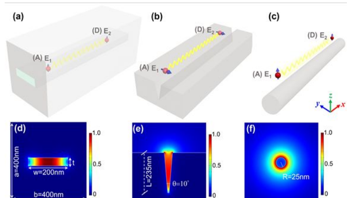
Figure 1 - Geometry of the proposed (a) ENZ plasmonic waveguide and two alternative plasmonic waveguides: (b) V-shaped groove and (c) cylindrical nanorod. All the presented waveguides are made of silver. A pair of two-level emitters [the donor (D) and acceptor (A)] are placed inside the nanochannel or along the different plasmonic waveguide structures. The lower panels (d)-(f) display the normalized fundamental mode distributions in the transverse cross section ( yz -plane) at the same wavelength \lambda = 1018\text{nm} and the geometry dimensions of each waveguide.
