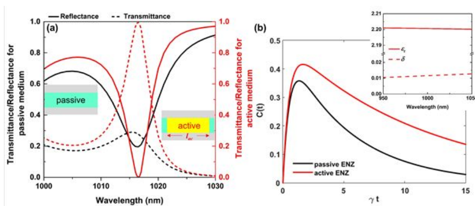
Figure 6 – (a) Transmittance and reflectance of the plasmonic waveguide in the vicinity of the ENZ resonance with (red) and without (black) gain. The left inset is the geometry of the passive ENZ plasmonic waveguide, and the right inset represents the active ENZ plasmonic waveguide. (b) Transient concurrence between the two qubits in the passive (black) and active (red) ENZ nanowaveguides for a fixed inter-qubits separation distance d = 900 nm. Inset: The Lorentz permittivity model of the realistic active dielectric material loaded inside the ENZ waveguide.
