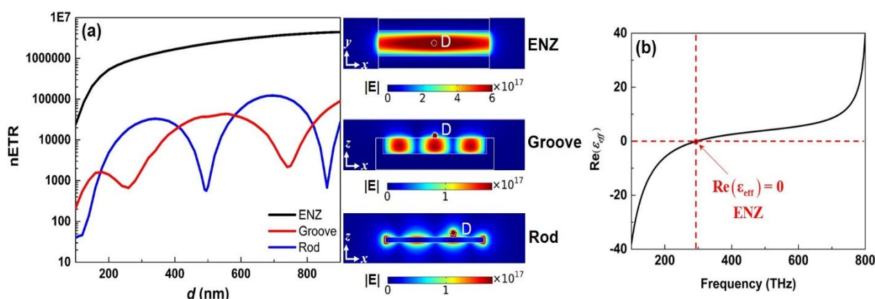
Figure 2 – (a) The computed nETR values as a function of the separation distance d between the donor-acceptor pair in the cases of the ENZ, finite groove, and cylindrical rod plasmonic waveguides (see Fig. 1 for the specifications of the waveguide geometries). We assume the location of the acceptor to be fixed in the beginning of the waveguide channel while the donor position is being continuously moved along the x -axis. Right insets: The static electric field patterns when the donor is placed in the center (ENZ, groove) or slightly to the right off the center (rod) of each waveguide. (b) The real part of the effective permittivity of the ENZ plasmonic waveguide versus the incident wave frequency. A near zero effective permittivity is achieved at the cutoff frequency around 295 THz (corresponding to \lambda = 1016 nm).
