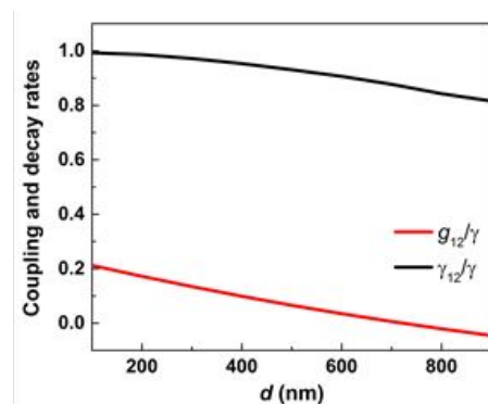
Figure 4 - Normalized decay rate \gamma_{12}/\gamma and dipole-dipole interaction g_{12}/\gamma of two qubits placed inside the ENZ plasmonic waveguide as a function of the emitters' separation distance d . The obtained values are normalized to \gamma , which is the spontaneous emission decay rate of a single emitter placed in the waveguide.
