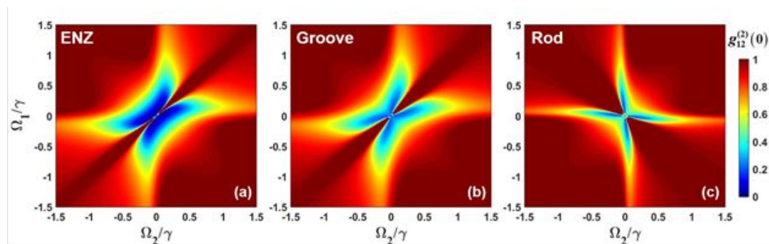
Figure 9 - Zero-delay correlations vs pumping intensities for the cases of (a) ENZ, (b) groove, and (c) cylindrical rod plasmonic waveguides, using the same parameters reported before in Figs. 7(d)-(f). The emitters' separation distance is fixed to d=700\text{nm} in these results.
