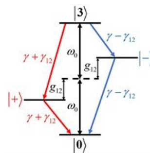
Figure 3 - Collective states diagram of two identical emitters. The two identical qubits (emitters) are located at equivalent positions with respect to the plasmonic system and have identical orientations.
