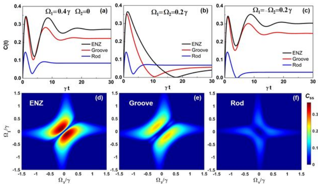
Figure 7 - Time dependence of the concurrence between two qubits pumped by (a) asymmetric, (b) symmetric, and (c) antisymmetric pumping. Lower panels (d)-(f): Steady state concurrence vs pumping intensities for the cases of (d) ENZ, (e) groove, and (f) cylindrical rod plasmonic waveguides. The emitters' separation distance is fixed to d = 700\text{nm} in these results.
