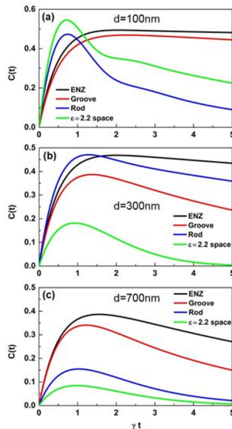
Figure 5 - Transient concurrence between the two qubits placed in the ENZ (black lines), groove (red lines), and cylindrical rod (blue lines) nanowaveguides for three inter-qubits separation distances: (a) d = 100 nm, (b) d = 300 nm, and (c) d = 700 nm. The green lines refer to the qubits placed in a dielectric bulk medium (no waveguide) with relative permittivity \epsilon = 2.2 .
