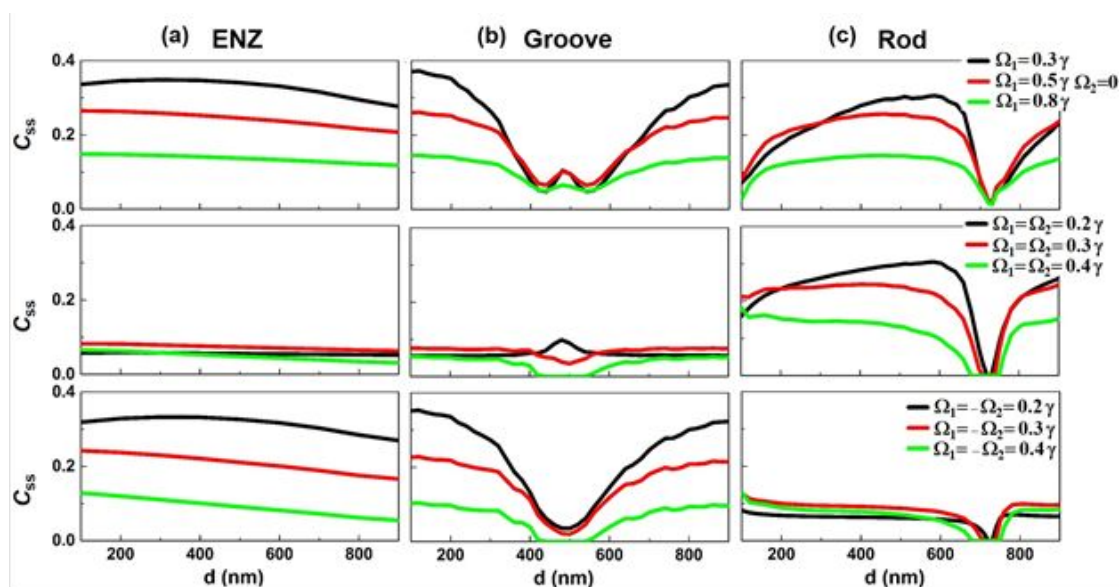
Figure 8 - Steady state concurrence as a function of the qubits' separation distance monitored at the normalized time \gamma t = 70 for the cases of (a) ENZ, (b) groove, and (c) cylindrical rod plasmonic waveguides by using the asymmetric, symmetric, and antisymmetric pumping.
