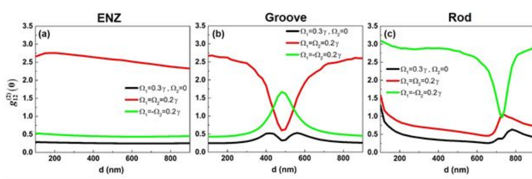
Figure 10 - A potential experimental validation of the qubit-qubit entanglement characterized by the second-order photon correlation function at zero time delay as a function of the emitters' separation distance for the cases of (a) ENZ, (b) groove, and (c) cylindrical rod plasmonic waveguides by using asymmetric, symmetric, and antisymmetric pumping.
