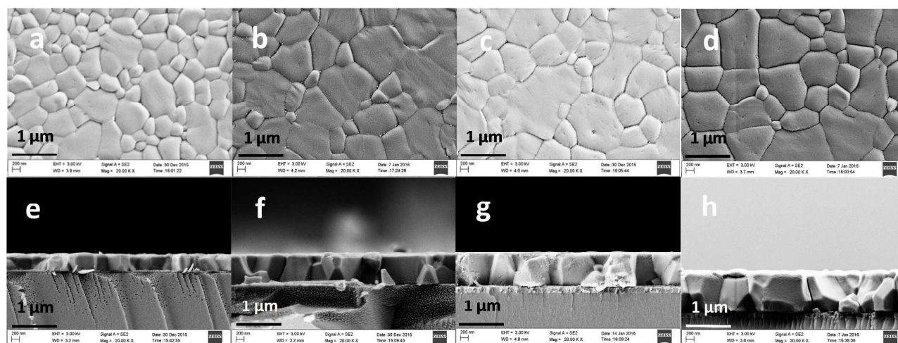
Figure 8 Top-view (a-d) and cross-sectional (e-h) SEM image of \text{CH}_3\text{NH}_3\text{PbI}_3 perovskite films prepared with different thickness: (a, e) \sim 420 nm, (b, f) \sim 650 nm, (c, g) \sim 850 nm, (d, h) \sim 1020 nm.
