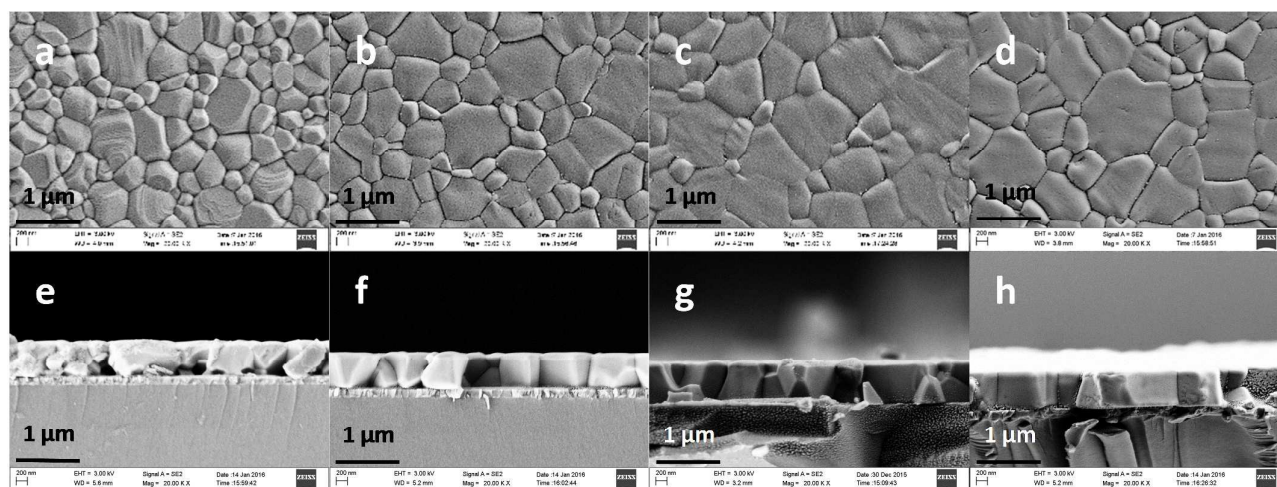
Figure 2 Top-view (a-d) and cross-sectional (e-h) scanning electron microscopy image of \text{CH}_3\text{NH}_3\text{PbI}_3 perovskite films prepared using different pre-annealing temperatures: (a, e) without pre-annealing step, (b, f) 80 °C, (c, g) 100 °C, (d, h) 120 °C.
