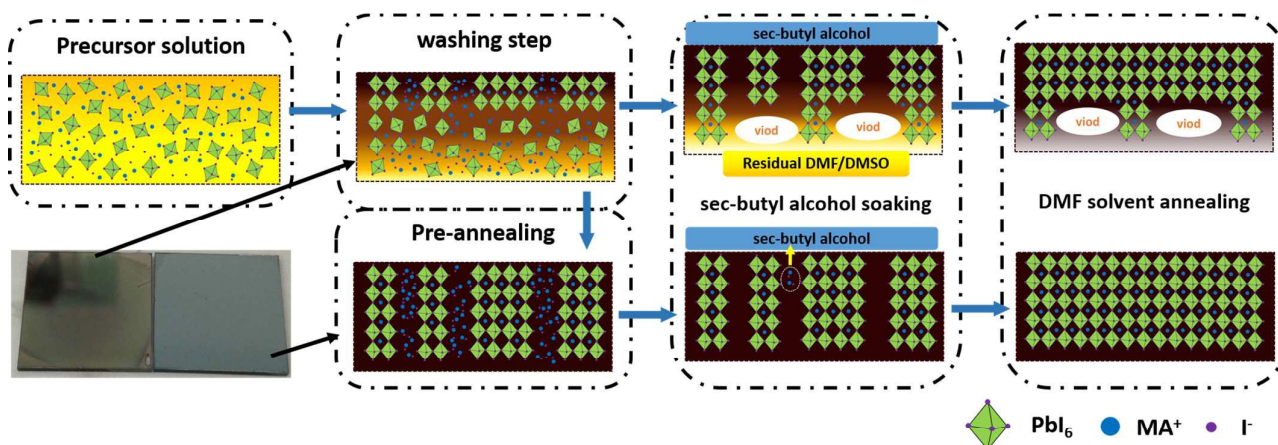
Figure. 4 Schematic illustration of the perovskite crystal growing process, including washing, pre-annealing, soaking, and post-annealing steps.
