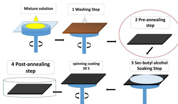
Figure 1 Schematic illustration of the fabrication procedure including washing, pre-annealing, soaking, and post-annealing steps.
