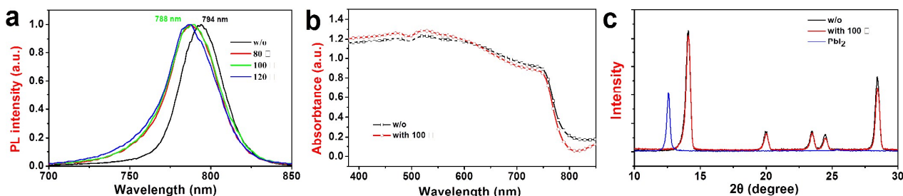
Figure 3 (a) Normalized photoluminescence spectra (PL) of perovskite thin films prepared with different pre-annealing temperature. An excitation light of 325 nm irradiated on the film from the air side, and the PL signal was also collected from the air side. (b) Absorption spectra and (c) X-ray diffraction patterns of \text{CH}_3\text{NH}_3\text{PbI}_3 perovskite films prepared with and without pre-annealing step. The \text{CH}_3\text{NH}_3\text{PbI}_3 films were spun on the surface of an ITO/PEDOT: PSS layer to ensure the identical condition to the working device.
