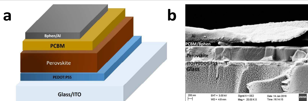
Figure. 5 (a) Schematic device structure of perovskite solar cell; the devices were structured as ITO/PEDOT: PSS/ \text{CH}_3\text{NH}_3\text{PbI}_3 /PCBM/Bphen/Al. (b) Cross-sectional scanning electron microscopy image of the full perovskite solar cell under 100^\circ\text{C} pre-annealing conditions.
