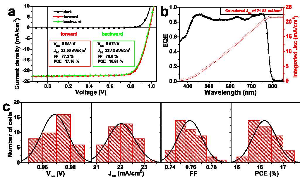
Figure 7 (a) J-V curves and (b) external quantum efficiency (EQE) spectrum together with EQE data based integrated short-circuit current density ( J_{sc} ) for the best performing perovskite solar cell. The J-V data were collected under AM 1.5G one sun illumination ( 100 \text{ mW/cm}^2 ). (c) Histograms of J_{sc} , open-circuit voltage ( V_{oc} ), fill factor (FF), and power conversion efficiency (PCE) of 40 cells, respectively.
