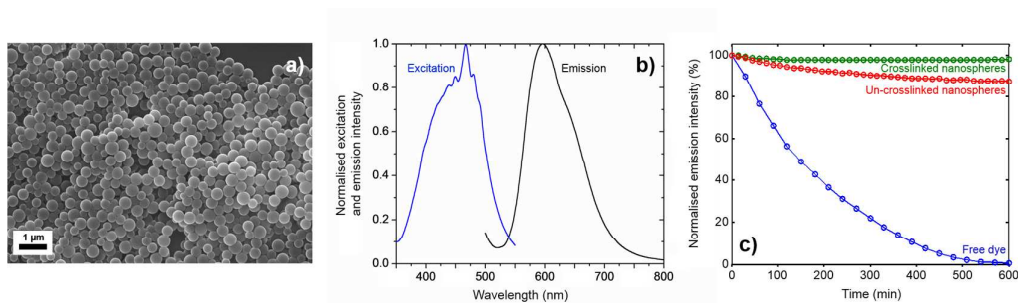
Figure 2: a) Representative SEM image showing fully formed and crosslinked nanospheres, \sim 300 nm in diameter prepared from water. b) Normalised photoluminescence excitation and emission spectra for the crosslinked nanospheres in water. c) Normalised emission intensity versus time for crosslinked and non-crosslinked nanospheres in water under constant excitation at 450 nm. Also shown is equivalent data for the free dye in de-aerated ethanol.
