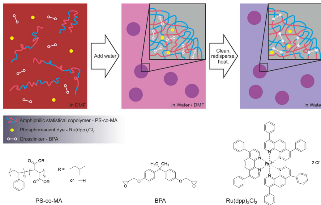
Figure 1: Schematic illustrating the co-precipitation/crosslinking process used to prepare the phosphorescent polymer nanospheres (top), and the molecular structures of the constituent materials (bottom).
