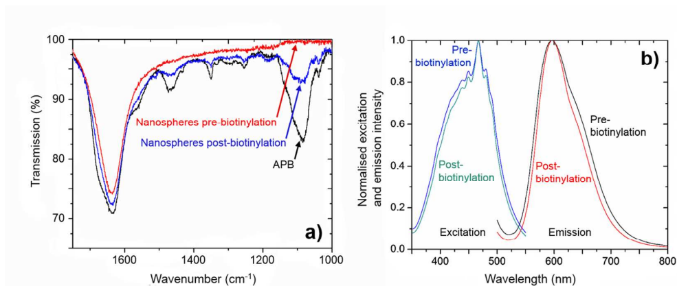
Figure 4: a) FTIR spectra for nanospheres after biotinylation and cleaning (blue). Also shown for comparison are the spectra of the selected biotin derivative (APB, black) and the unfunctionalised nanospheres (red) prior to the biotinylation procedure. b) Normalised photoluminescence excitation and emission spectra of nanospheres before and after biotinylation. In each case minimal changes in peak shape and location are seen.
