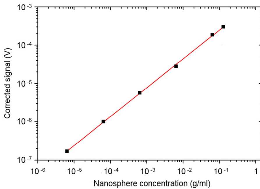
Figure 3: Time-gated signal intensity versus nanosphere concentration for crosslinked dye-doped nanospheres dispersed in water.
