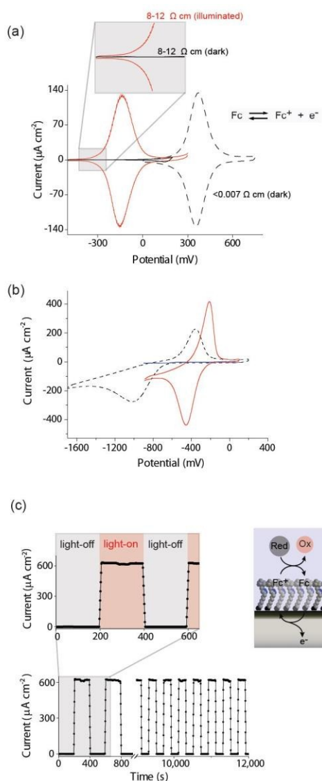
Fig. 2 (a) A cyclic voltammogram (CV) (dash black line) in aqueous 1.0 M HClO 4 at highly doped (<math><0.007 \Omega \text{ cm}</math>, dopant concentration, N_A > 8 \times 10^{18} \text{ cm}^{-3} ) p-Si electrodes that behave electrochemically similar to metals. A CV of a poorly doped n-Si electrode (8–12 \Omega \text{ cm} , N_D, \sim 4.5 \times 10^{14} \text{ cm}^{-3} ) in the dark (solid black line) and light (solid red line) at 642 nm, \sim 300 \text{ mW cm}^{-2} . (b) CVs (dash black line) at highly doped p-Si electrodes (<math><0.003 \Omega \text{ cm}</math>, dopant concentration, N_A \sim 1 \times 10^{19} \text{ cm}^{-3} ) and poorly doped p-Si electrode (substrate: 1–10 \Omega \text{ cm} , N_A, \sim 8 \times 10^{14} \text{ cm}^{-3} ; illumination: 642 nm, \sim 300 \text{ mW cm}^{-2} ) to a surface bound anthraquinone at pH 10.1 in the dark (solid blue line) and light (solid red line). (c) Amperometric trace demonstrating the switching ON and OFF of heterogeneous catalysis promoted by surface-bound ferrocene from an n-Si electrode to an aqueous. The n-Si electrode is poised at +0.2 V versus Ag|AgCl|3M NaCl and 1 mM ferrocyanide [\text{Fe}(\text{CN})_6]^{4-} in solution recycles the ferricinium back to ferrocene with modulation of the illumination (0.1 M KNO 3 at pH 7; substrate: 8–12 \Omega \text{ cm} ; illumination: 527 nm, \sim 1.77 \text{ mW cm}^{-2} , modulation is 200 s ON and 200 s OFF).
