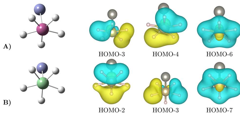
Figure 4: Anionic \text{TMZnH}_5^- polyhydride complexes. Figure A) \text{IrZnH}_5^- molecule along with the most relevant MOs of \text{IrZnH}_5^- , B) \text{OsZnH}_5^- molecule and its most relevant MOs of \text{OsZnH}_5^- are shown. Ir, Os, Zn and H are represented with pink, green, violet and white spheres respectively.
