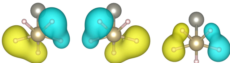
Figure 5: AdNDP result for \text{OsZnH}_5^- complex.
