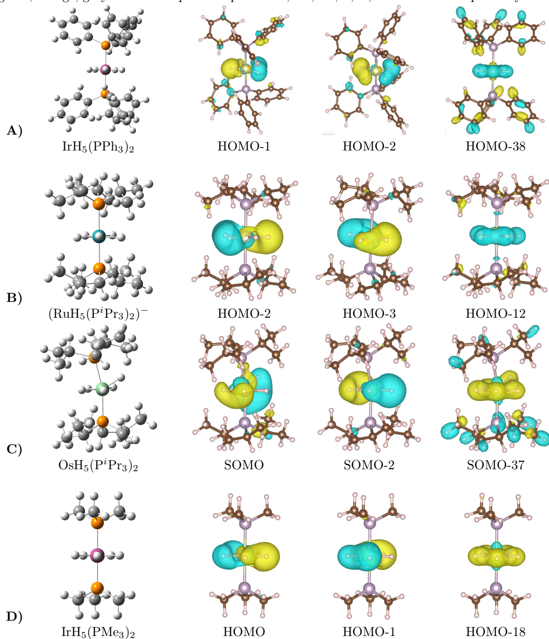
Figure 1: Transition-metal hydride complexes along with the most relevant MO's in each case. The pink, turquoise, green, orange, gray and white spheres represent Ir, Ru, Os, P, C, and H atoms respectively.
