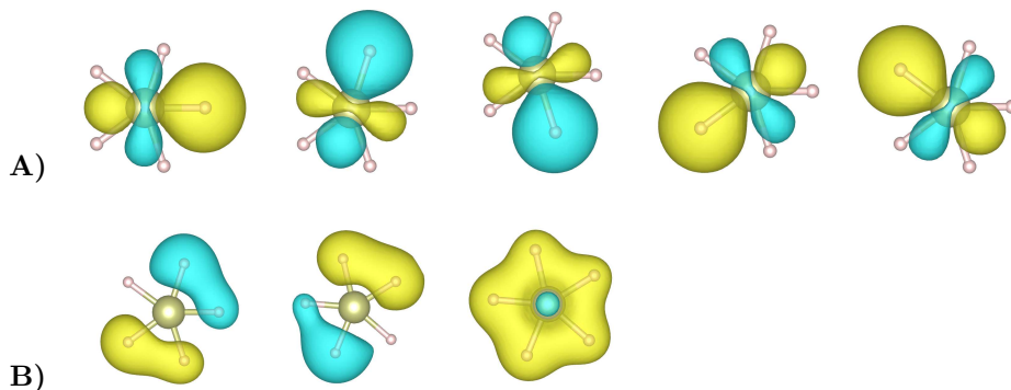
Figure 2: The two different AdNDP bonding pictures for IrH 5 .
