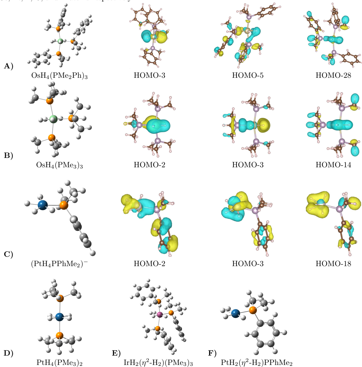
Figure 3: Transition-metal hydride complexes. The pink, green, blue orange, gray and white spheres represent Ir, Os, Pt, P, C, and H atoms respectively.
