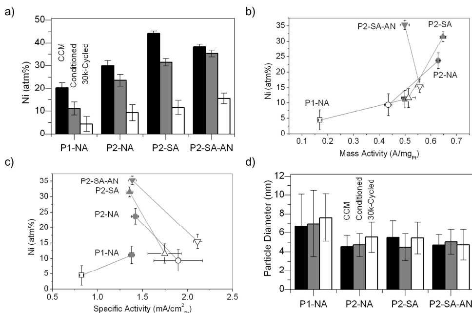
Figure 3. (a) EPMA-determined Ni atomic percentages, where black, dark grey, and white represent pristine CCM, conditioned and 30k-cycled MEA, respectively. (b) and (c) The average Ni atomic percentages determined by EPMA plotted against the mass and specific activities of the MEAs, respectively. (Dark grey: conditioned; white: 30k-cycled.) From (a) to (c), the activity error bars represent the standard deviation of activity measurements among at least 4 MEA samples, while the Ni-content error bars represent the standard deviation of EMPA measurements among at least 3 different locations. (d) TEM-determined mean particle size from different MEAs, where black, dark grey and white represent pristine CCM, conditioned MEA and 30k-cycled MEA, respectively. For each sample over 100 particles were measured to get the average size and the error bars represent the standard deviation.
