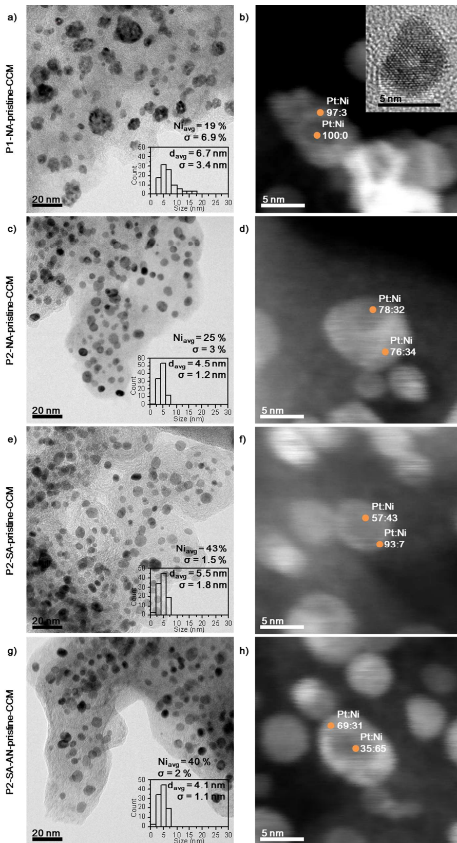
Figure 4. Bright-Field diffraction contrast TEM images with PSDs, Ni atomic percentages determined from parallel-beam EDS (left) and HAADF STEM images with point-mode EDS (right) from catalyst particles taken from pristine CCMs. (a) and (b) P1-
