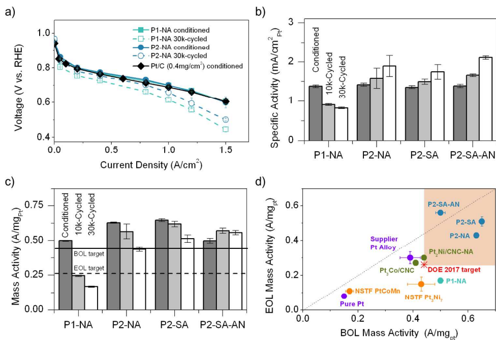
Figure 2. (a) Fuel cell polarization curves of MEAs with P1-NA and P2-NA cathodes at different aging stages (conditioned and 30k-cycled), and of conditioned Pt as a reference. The catalyst loadings were 0.1 and 0.4 mg Pt /cm 2 for the dealloyed PtNi and commercial Pt catalysts, respectively. Testing conditions of anode/cathode were H 2 /air, 100/100% RH, 170/170 kPa abs back pressure, and stoichiometric coefficient of 1.5/2, respectively. (b) Specific activity and (c) mass activity of the catalysts made using P1 and P2. The activities were measured at 0.9 V (vs. RHE) from the H 2 /O 2 polarization curve collected at 80°C, 100 % relative humidity (RH) and 150 kPa abs after high frequency resistance-correction, where dark grey, light grey and white represent conditioned, 10k-cycled and 30k-cycled MEA, respectively. From (a) to (c) the error bars represent the standard deviations of activity measurements among at least 4 MEA samples. (d) The end-of-life (EOL, 30k-cycled MEA) vs. beginning-of-life (BOL, conditioned MEA) mass activity for catalysts from this work and from previous work on MEAs: 3M NSTF PtCoMn, NSTF Pt 3 Ni 7 , 61 Pt 3 Co/CNC and Pt 2 Ni/CNC, 62 Supplier Pt Alloy and pure Pt. 52, 63 The solid and dash horizontal lines in (b) and the red star and the green square regions represent the DOE 2017 PEMFC cathode catalyst targets for BOL mass activity (0.44 A/mg Pt ) and EOL mass activity (0.26 A/mg Pt ), 51 respectively.
