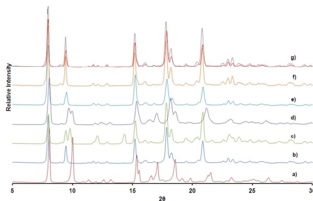
Fig. 10. a) PXRD traces of a) 1d-methanol , b) 1d-butanol , c) obtained after soaking crystals in a solvent mixture of n -butanol and methanol for several weeks, d) obtained after exposing polycrystalline activated phase, 1d to vapours derived from the 1:1 liquid mixture of n -butanol and methanol for 6 hours, e) after 24hrs exposure to vapours of the liquid mixture, f) pxrd obtained after 72hrs of exposure to solvent mixture vapour and g) overlay of a) in red and f) in grey.
