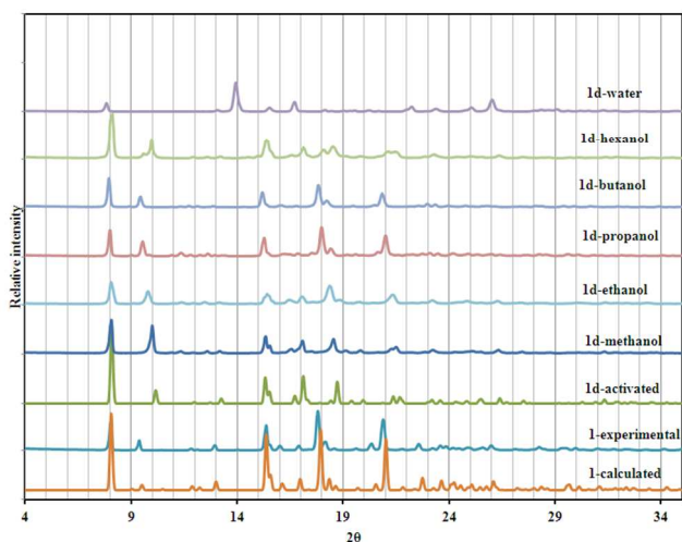
Fig.5. PXRD of 1 , 1d and several solvated forms of 1d at room temperature.
