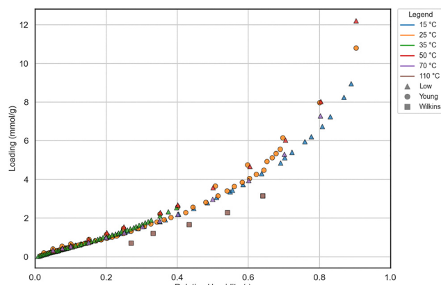
Fig. 3 Unary H 2 O adsorption isotherms, covering multiple temperatures and sources.
