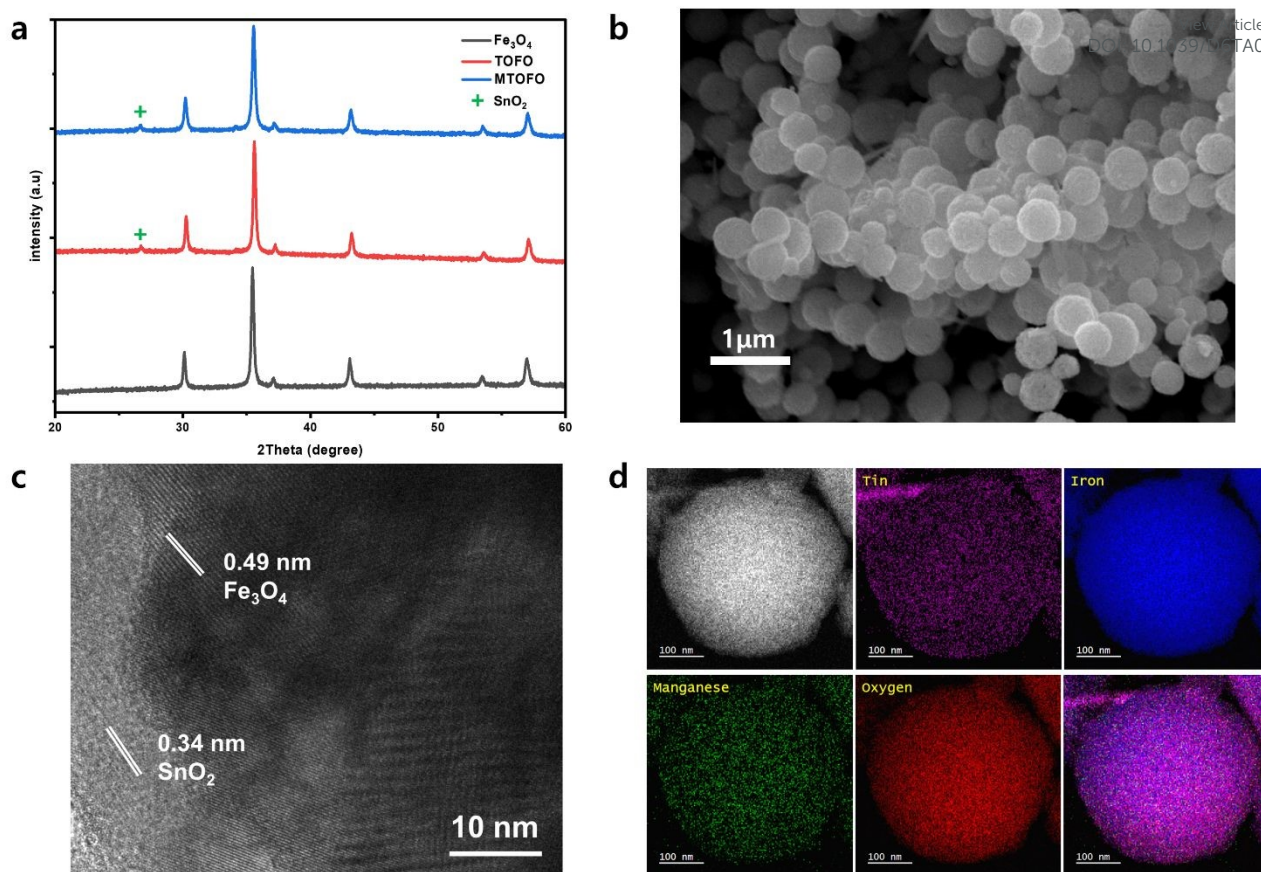
Fig. 1 Characterization of crystal structure and Morphology: (a) XRD patterns of \text{Fe}_3\text{O}_4 , TOFO, MTOFO. (b) SEM image of MTOFO. (c) HR-TEM image of MTOFO. (d) HAADF-STEM images of MTOFO and EDS corresponding elemental and mixed mapping.
