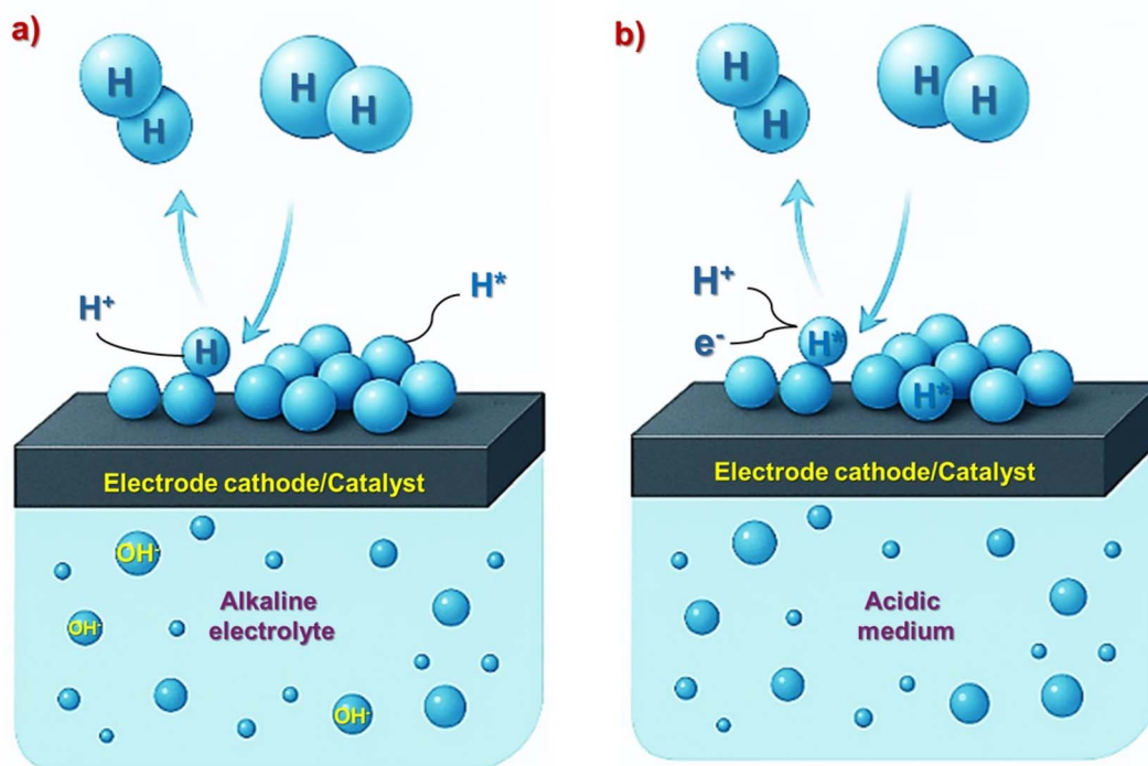
Fig. 1 Schematic illustration of the HER mechanism in alkaline medium (a) and acidic medium (b).
