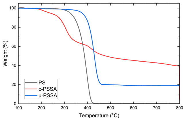
Fig. 3 TGA thermograms of all three polymers, heated at a heating rate of 10\text{ }^{\circ}\text{C min}^{-1} from 100 to 800\text{ }^{\circ}\text{C} under a nitrogen atmosphere (flow rate: 25\text{ mL min}^{-1} ).
