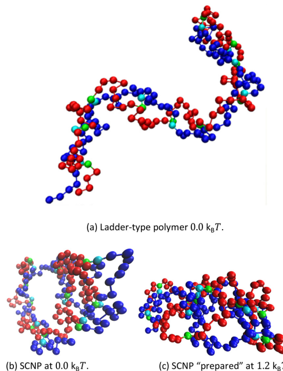
Fig. 4 Simulation snapshots of a ladder-type polymer with 0.0 k_B T interaction energy \epsilon between the beads of the two different ladder spars (this ideal ladder was taken as a structural model for the simulation, meaning that the connectivity was “presynthesized” prior to the MC simulation) (a) and two examples for SCNPs equilibrated and depicted at 0.0 k_B T , but either “synthesized” at 0.0 k_B T (b) or at 1.2 k_B T (c) (for the later cases, the connectivity was a result of the in silico synthesis during our MC simulations).
