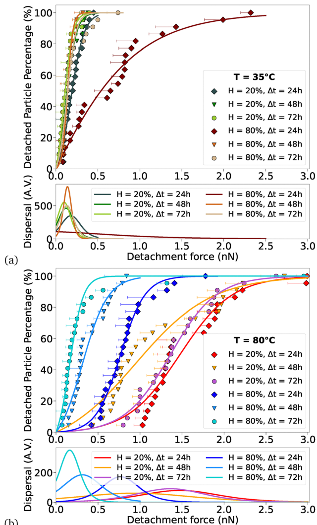
Fig. 4 Effect of humidity and drying time variation ( \Delta t ) on detachment force under constant temperatures of (a) 35\text{ }^{\circ}\text{C} and (b) 80\text{ }^{\circ}\text{C} . Solid lines in the main plot represent fitted logistic functions.
