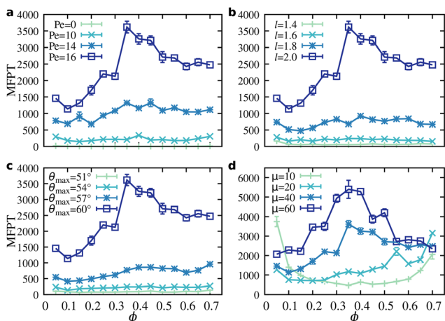
Fig. 6 Lifetime of the motile state indicated by the mean-first passage time (MFPT) as a function of the packing fraction for different values of the active force magnitude Pe , the rod length l , the maximum angle \theta_{\max} , and the mobility \mu of each disk forming the active rod. For each plot, the fixed parameters are as follows: (a) l = 2 , \theta_{\max} = 60^\circ , \mu = 40 ; (b) Pe = 16 , \theta_{\max} = 60^\circ , \mu = 40 ; (c) Pe = 16 , l = 2 , \mu = 40 ; (d) Pe = 16 , l = 2 , \theta_{\max} = 60^\circ . The error bars indicate the standard deviations, and the lines are to guide the eye.
