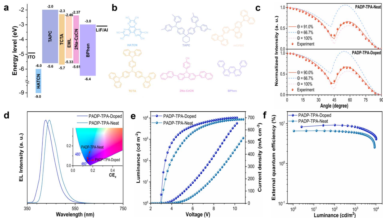
Fig. 5 (a) Doped device structure; (b) structure of the functional layers; (c) measured horizontal transition dipole moment ratios of PADDP-TPA in the neat film and doped film. (d) PADDP-TPA pure film EL spectrum and EL spectrum of the device with 20 wt% PADDP-TPA doped in the mCPBC host; the inset shows the CIE coordinates of the EL spectra. (e) Current density–voltage–luminance characteristics of the devices. (f) The external quantum efficiency versus the current density.
