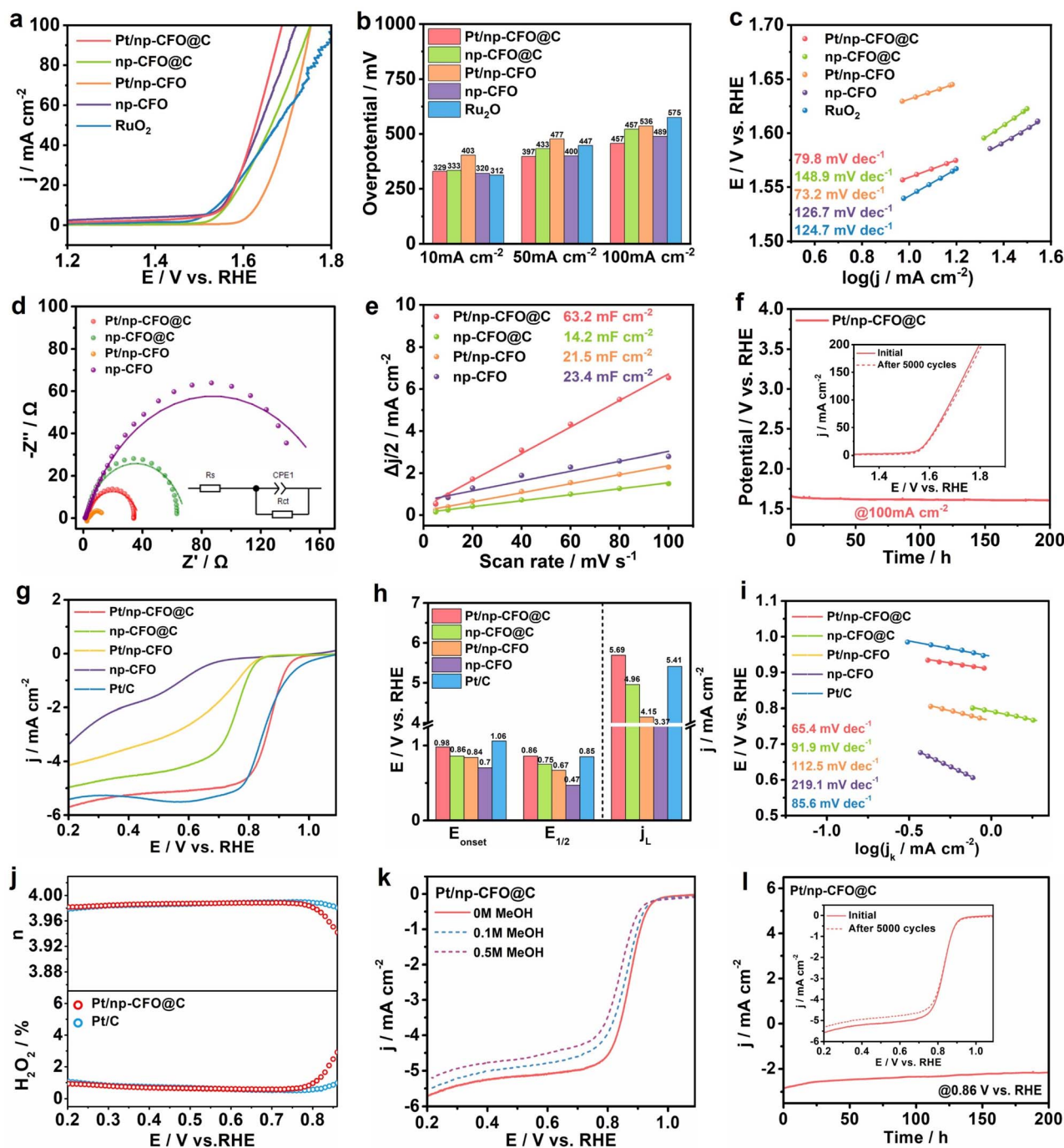
Fig. 4 OER performances: (a) LSV curves; (b) a comparison of \eta_{10} , \eta_{50} and \eta_{100} ; (c) Tafel slopes; (d) Nyquist plots; (e) C_{dl} values; and (f) the CP profile at 100 \text{ mA cm}^{-2} ; the inset shows LSV curves of Pt/np-CFO@C before and after ADT. ORR performances: (g) LSV curves; (h) a comparison of E_{onset} , E_{1/2} and j_L ; (i) Tafel slopes; (j) electron transfer numbers and \text{H}_2\text{O}_2 yields on Pt/np-CFO@C and Pt/C derived from RRDE testing; (k) methanol tolerance of Pt/np-CFO@C; and (l) the CA profile at 0.86 \text{ V vs. RHE} ; the inset shows LSV curves of Pt/np-CFO@C before and after ADT.
