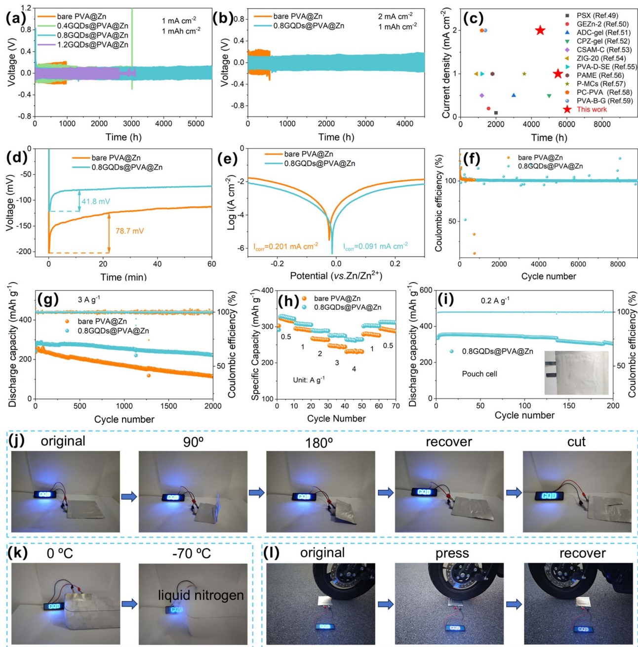
Fig. 3 Electrochemical performance of the GQD-modified hydrogel electrolyte. Cycling performance of Zn||Zn symmetric cells with bare PVA@Zn and 0.8GQDs@PVA@Zn at 1 \text{ mA cm}^{-2} (a) and 2 \text{ mA cm}^{-2} (b). (c) Comparison of the cycling properties of 0.8GQDs@PVA@Zn with those in other reports. (d) Nucleation overpotential curves for zinc nucleation. (e) Tafel curves of the Zn anode. (f) Coulombic efficiency of Zn||Cu batteries. (g) Cycling performance of Zn||NVO full cells at 3 \text{ A g}^{-1} . (h) Rate capability at different current densities from 0.5 to 4 \text{ A g}^{-1} . (i) Cycling performance of the Zn||NVO pouch cell using 0.8GQDs@PVA@Zn at 0.2 \text{ A g}^{-1} . Photographs of the pouch cell using 0.8GQDs@PVA@Zn as the electrolyte, driving an LED light under bending, shearing (j), freezing (k), and compression (l) conditions.
