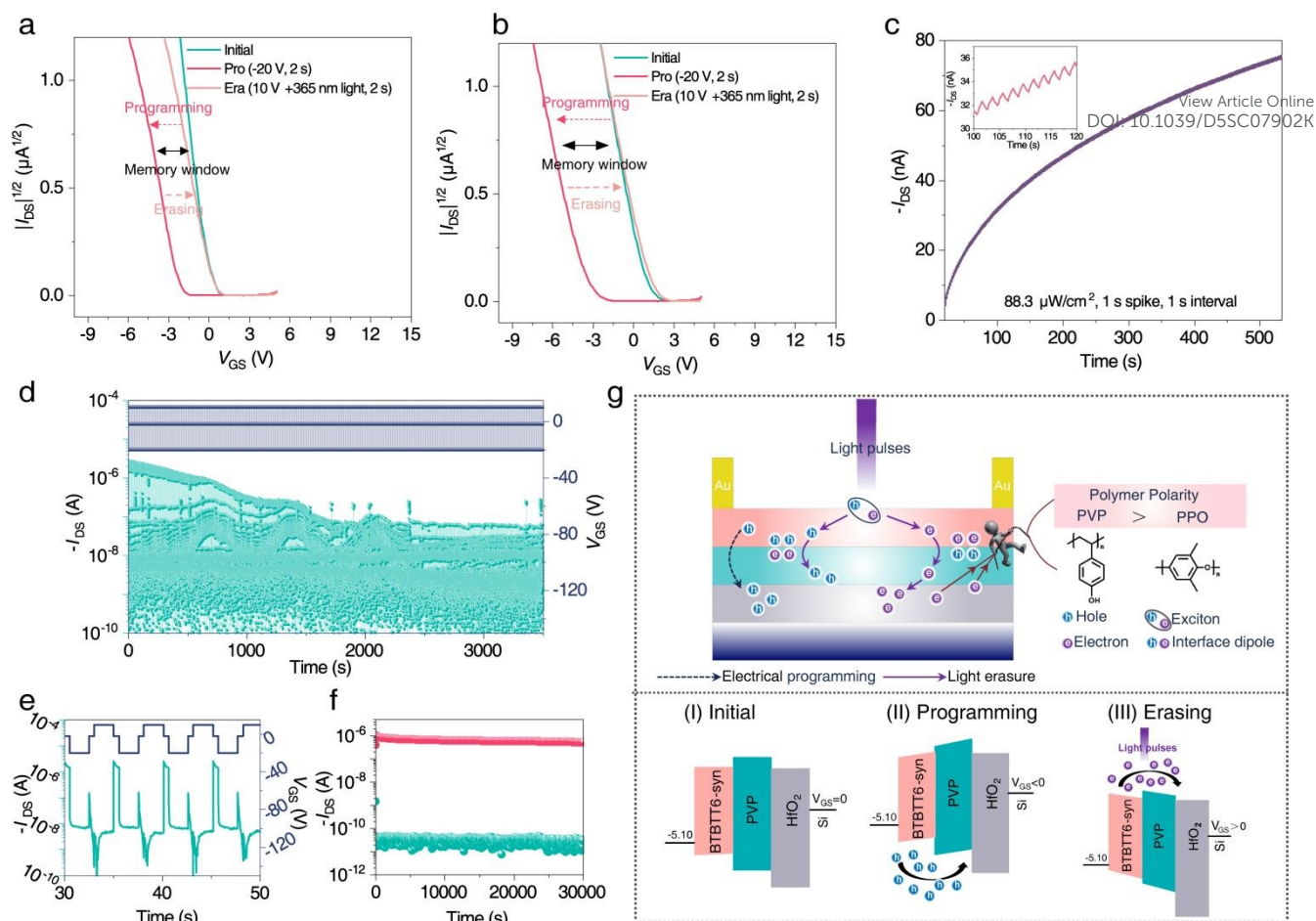
Fig. 2. Transfer curves corresponding to the initial state, electrical-programmed state, and light-erased state of (a) PVP/HfO 2 -based and (b) PPO/HfO 2 -based device. Electrical-programmed state was conducted at V_{GS} = -20 V with t_{\text{spike}} = 2 s, and light-erased state was achieved under a 365 nm light pulse ( t_{\text{spike}} = 2 s) at V_{GS} = 10 V. (c) Multilevel memory of PPO/HfO 2 -based device by multiple light pulse stimulations; the inset is corresponding magnified curves. (d) Endurance characteristics of the PVP/HfO 2 -based device over 700 P/E cycles. (e) Detailed curves of the endurance characteristics of the PVP/HfO 2 -based device, programmed at V_{GS} = -20 V with t_{\text{spike}} = 2 s, erased by a 365 nm light pulse ( t_{\text{spike}} = 2 s) at V_{GS} = 10 V. (f) Retention characteristics of electrical-programmed state and light-erased state of PVP/HfO 2 -based device. (g) Working mechanism of electrical-programmed state and light-erased state in the PVP/HfO 2 -based device.
