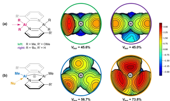
Figure 12 Topographic steric maps showing the steric pressure exerted on each aluminium centre: (a) by the ring system in the neutral precatalysts 1c and 1d (left and right, respectively; viewed on the plane of the ring from the direction of the alkyl groups); (b) by the ring system in the active cationic catalyst 2a (viewed from the direction of the terminal methyl) (left) or by the entire ligand scaffold (including terminal alkyls, viewed from the direction of the incoming substrate) (right). The scale of the isocontours of altitude from the Al centre range between \pm 3.5 Å.
