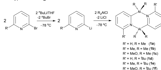
Scheme 3 Synthesis of Al(III) dimers of the type (2-py') 2 (2-py' = 6-substituted pyridyl), the precatalysts used in polymerisation and cyclotrimerisation in the current study, including the compound numbering scheme.
