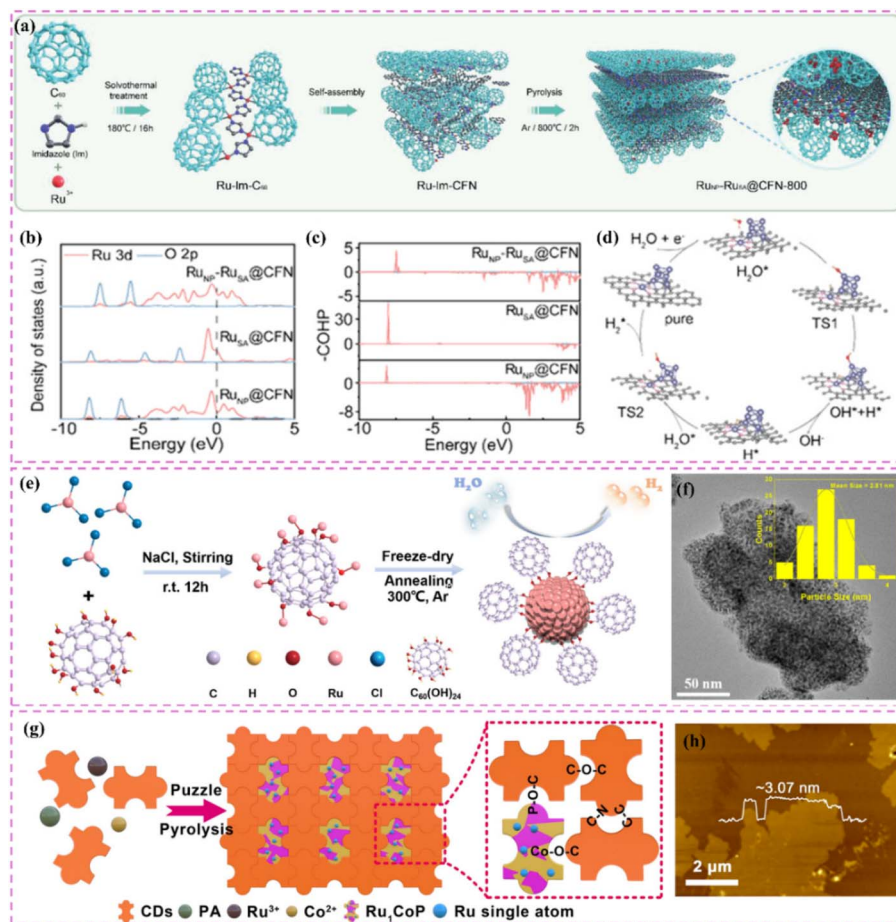
Fig. 7 (a) Schematic illustration of the synthetic process of RuNP-RuSA@CFN-800. (b) DOS and (c) COHP diagram for RuNP-RuSA@CFN, RuSA@CFN and RuNP@CFN. (d) Proposed possible HER mechanism for RuNP-RuSA@CFN in alkaline medium. Reproduced with permission from ref. 120. Copyright 2023, Wiley-VCH. (e) Synthesis Procedure for Ru-OC 60 -300. TEM images of Ru-OC 60 -300. The inset in (f) shows the particle size distribution of Ru NPs. Reproduced with permission from ref. 121. Copyright 2023, American Chemical Society. (g) Formation of Ru 1 CoP/CDs. (h) AFM image of Ru 1 CoP/CDs-1000. Reproduced with permission from ref. 122. Copyright 2021, Wiley-VCH.
