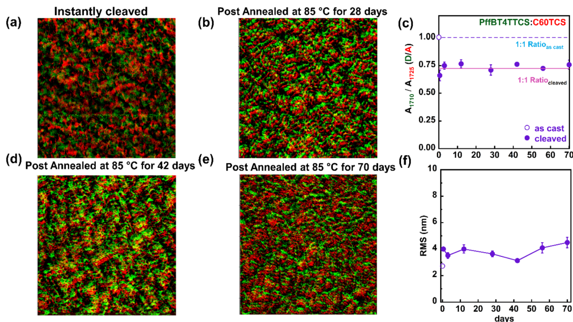
Fig. 4 Stability measurement of the active layer (PffBT4T-TCS : C60-TCS = 1 : 1) under continuous thermal annealing at 85 °C: (a) overlay image of the cleaved active layer immediately after thermal cleavage; (b) overlay image of the cleaved active layer after annealing at 85 °C for 28 days; (c) evolution of local chemical compositions for as-cast and cleaved active layer as a function of annealing time; (d) overlay image of the cleaved active layer after 42 days of annealing at 85 °C; (e) overlay image of the cleaved active layer after 70 days of annealing at 85 °C; (f) surface roughness as a function of annealing time. In all overlay images, green and red regions represent donor and acceptor, respectively.
