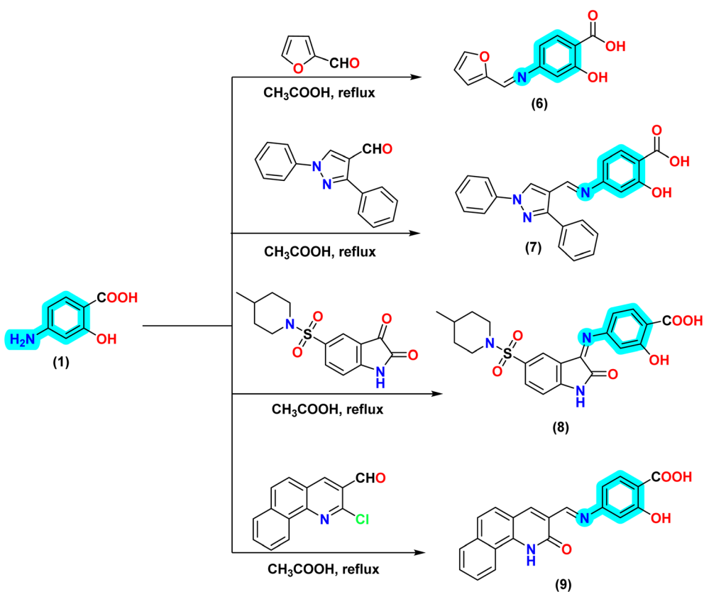
Scheme 2 Synthesis of new salicylic acid Schiff base derivatives incorporating heterocyclic fragments, including furan, pyrazole, 2-oxindoline, and benzo[h]quinoline derivatives.
