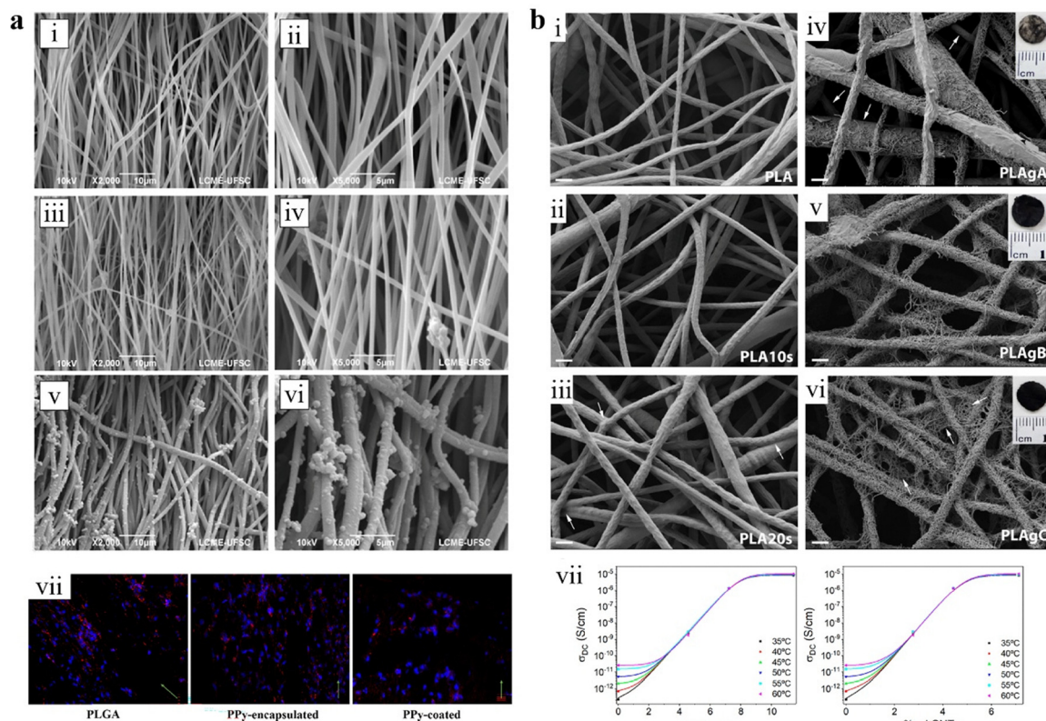
Fig. 12 Electrical conductivity and cellular responses of electrospun PLA grafting membranes. (a) Scanning electron micrographs of PLGA (i) and (ii), poly(PPy)-encapsulated (iii) and (iv), and poly(PPy)-coated electrospun mats (v) and (vi). Fluorescence micrographs of PC12 cells after 7 days on PLGA, poly(PPy)-encapsulated, and poly(PPy)-coated electrospun mats (vii). The blue staining was conducted by using 4',6-diamidino-2-phenylindole, which labels cell nuclei, and the red staining used phalloidin, which shows the actin cytoskeleton. Reprinted with permission from ref. 240. Copyright 2025, American Chemical Society. (b) Scanning electron micrographs and photographs (insets) of membranes and characterization of their fibre diameter before and after CNTs grafting: a nontreated electrospun PLA membrane (i), an electrospun PLA membrane treated with 30% H 2 SO 4 for 10 s (ii) and 20 s (iii). Electrospun PLA membrane grafted with CNTs after treated with 30% H 2 SO 4 for 10 s (iv), membrane grafted with CNTs after treated with 30% H 2 SO 4 for 10 s and subjected to water rinsing and drying (v), and membrane grafted with CNTs after treated with 30% H 2 SO 4 for 20 s and subjected to water rinsing and drying (vi). White arrows indicate areas where the CNTs fill the gaps between nanofibers. Electrical conductivity as a function of both mass fraction and volume fraction of CNTs present in the PLA membranes (vii). Reprinted with permission from ref. 358. Copyright 2023, American Chemical Society.
