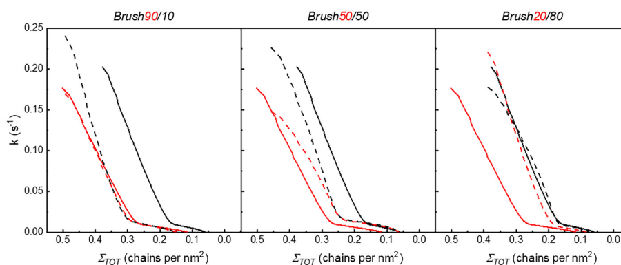
Fig. 5 k vs. \Sigma_{TOT} for the degrafting reaction of PS d85.2 -OH (dashed red line) and PS 13 -OH (dashed black line) in Brush90, Brush50 and Brush20. The curves representing k vs. \Sigma for the degrafting reaction in the single polymer brushes (see Fig. 3(b)) are also included as references, with a full red line for PS d85.2 -OH and a full black line for PS 13 -OH.
