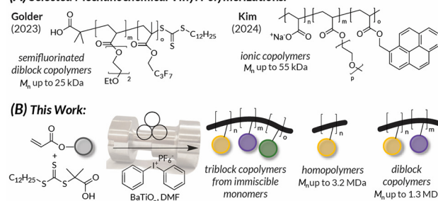
Fig. 1 (A) Previous work showcasing mechanochemically synthesized copolymers derived from immiscible vinylic monomers. 29,37 (B) This work features the ability MR-RAFT to access triblock copolymers from immiscible monomers and UHMW homopolymers and diblock copolymers.
