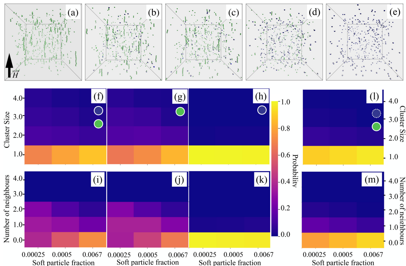
Fig. 3 (a–e) Typical room-temperature snapshots under a saturating magnetic field (field direction indicated on the left). The total volume fraction is 0.001. Configurations correspond to CoFe 2 O 4 :MnFe 2 O 4 ratios of (a) 1:0, (b) 3:1, (c) 1:1, (d) 1:2, and (e) 0:1. Green nanoparticles represent CoFe 2 O 4 , and blue nanoparticles represent MnFe 2 O 4 . (f–h) Heat maps showing the probability of finding clusters of specific sizes at different values of the magnetically soft particle volume fraction, under a saturating magnetic field: (f) both particle types in the mixtures are considered (PDE); (g) only magnetically hard particles are considered; (h) only magnetically soft particles are considered. (i–k) Heat maps of the probability for a particle to have a given number of nearest neighbours at different volume fractions, under a saturating magnetic field: (i) both particle types in the mixtures are considered (PDE); (j) only magnetically hard particles are considered; (k) only magnetically soft particles are considered. Panels (f) and (i) display results for all particles (both types), while panels (g) and (j) show only magnetically hard particles, and panels (h) and (k) only magnetically soft particles, as indicated by the green and blue circles, respectively. (l and m) (l) Probability of finding clusters of specific sizes, and (m) probability of a particle having a given number of nearest neighbours, at different volume fractions under a saturating magnetic field for mixtures of ideally superparamagnetic (blue, dashed outline) and magnetically hard (green) particles. Each plot is based on 50 statistically independent simulation snapshots. Clusters were identified using an energy-distance criterion: two particles belong to the same cluster if their separation is no more than 30% greater than the close-contact distance and if their dipolar interaction is attractive ( i.e. , negative). 61
