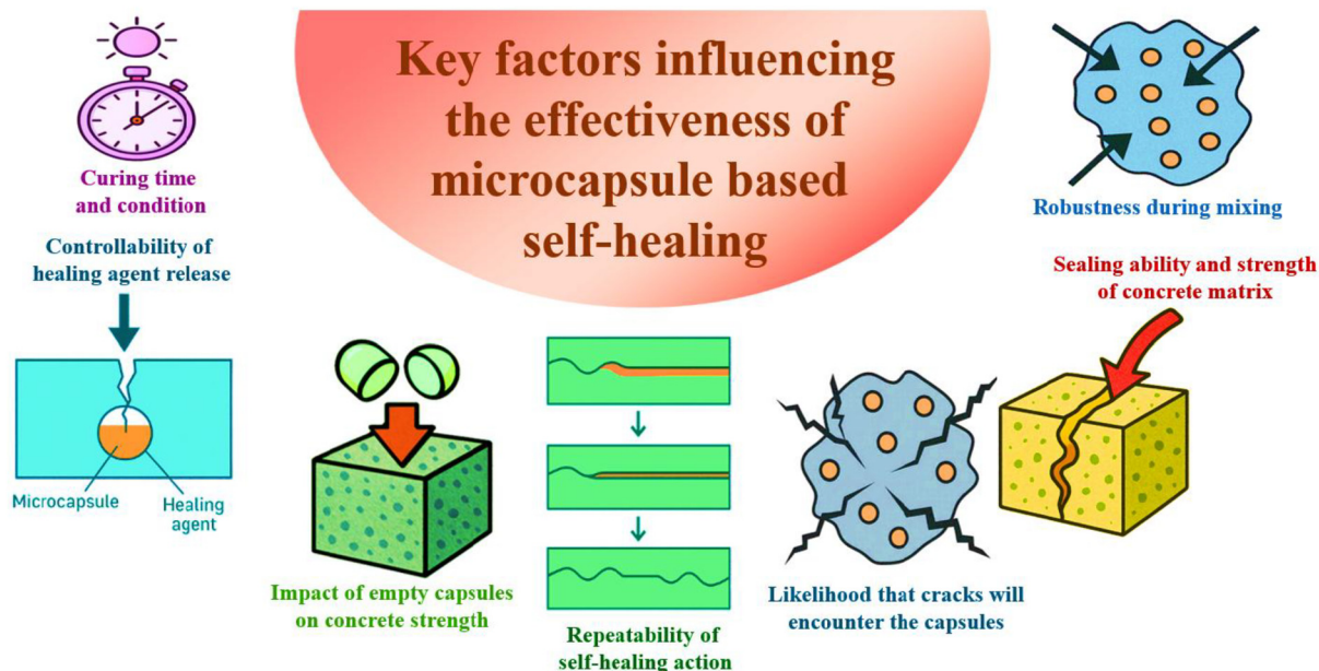
Fig. 2 Key factors influencing the effectiveness of microcapsule-based self-healing.
