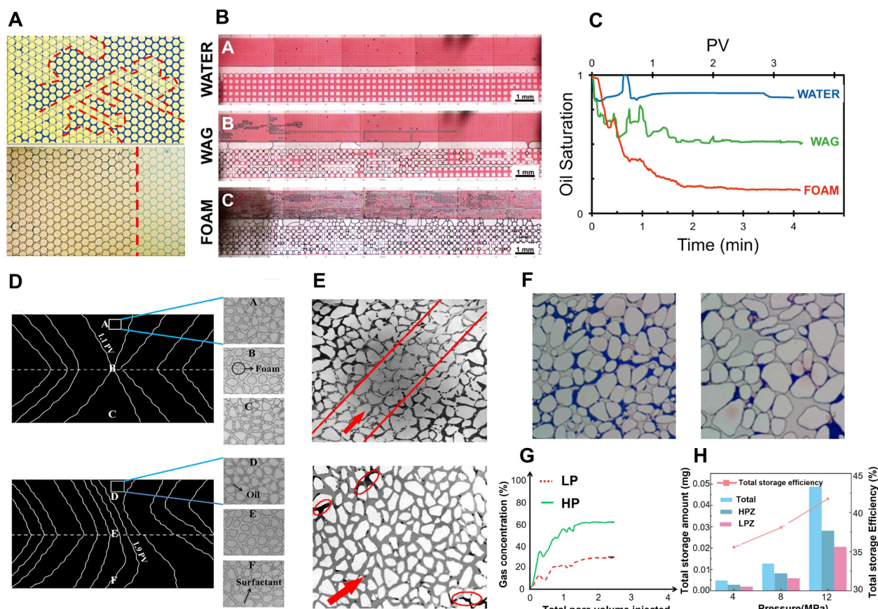
Fig. 13 Summary of displacement dynamics by foam in microfluidic models: (A) saline water displacement by \text{CO}_2 gas (yellow) showing viscous fingering (top) and by \text{CO}_2 foam with a stabilized front (bottom) at the flow rate of 100 \mu\text{L min}^{-1} in a quartz-etched porous medium (adapted with permission from Zheng et al. 218 Copyright © 2017 John Wiley & Sons). (B) Paraffin oil displacement by water, water alternating gas (WAG), and foam in a heterogeneous multi-layer microfluidic (PDMS) porous medium, demonstrating foam's superior oil recovery efficiency in all regions compared to water and WAG shown in (C) (adapted from Conn et al. 59 under CC-BY License). (D) Isopar V oil displacement by foam in 3D printed porous media placed horizontally (top) and vertically (bottom) to examine gravity effects on displacement patterns, highlighting gravity's impact on front propagation. In horizontal mode, gravity's impact is minimal, creating symmetrical fronts. In vertical mode, gravity override speeds up propagation in the lower region, leading to S-shaped fronts due to higher liquid saturation (adapted from Shojaei et al. 349 under CC-BY License). (E) Oil (black) displacement by water (top) and foam (bottom) in heterogeneous (glass-etched) media, showing foam's ability to mitigate fluid channeling and improve oil sweep efficiency (adapted with permission from Sun et al. 350 Copyright © 2014 American Chemical Society). (F) Residual oil (pink) after water then foam injection into heterogeneous porous media with (left) low and (right) high permeability that were laser-etched on glass substrates. Foam displaced the residual oil remaining after water flooding and reached over 90% oil recovery in both cases. Larger pore and throat sizes of the high permeable structure allowed higher gas saturation (adapted with permission from Wang et al. 311 Copyright © 2021 American Chemical Society). (G) Gas saturation vs. time (injected pore volume) during oil displacement by foam in a heterogeneous porous medium with two high and low permeable layers fabricated on a UV curable epoxy (NOA 81). Gas saturation is higher in the more permeable region due to greater opposing capillary pressures that prevent non-wetting gas from entering less permeable areas (adapted with permission from Xiao et al. 81 Copyright © 2018 American Chemical Society). (H) Gas storage vs. gas-injection pressure during oil displacement by gas in a heterogeneous (glass-etched) porous medium with high (HPZ) and low (LPZ) permeable zones. Higher pressures improved gas storage by overcoming capillary resistance, allowing greater gas saturation in more permeable areas (adapted with permission from Qian et al. 196 Copyright © 2025 Elsevier).
