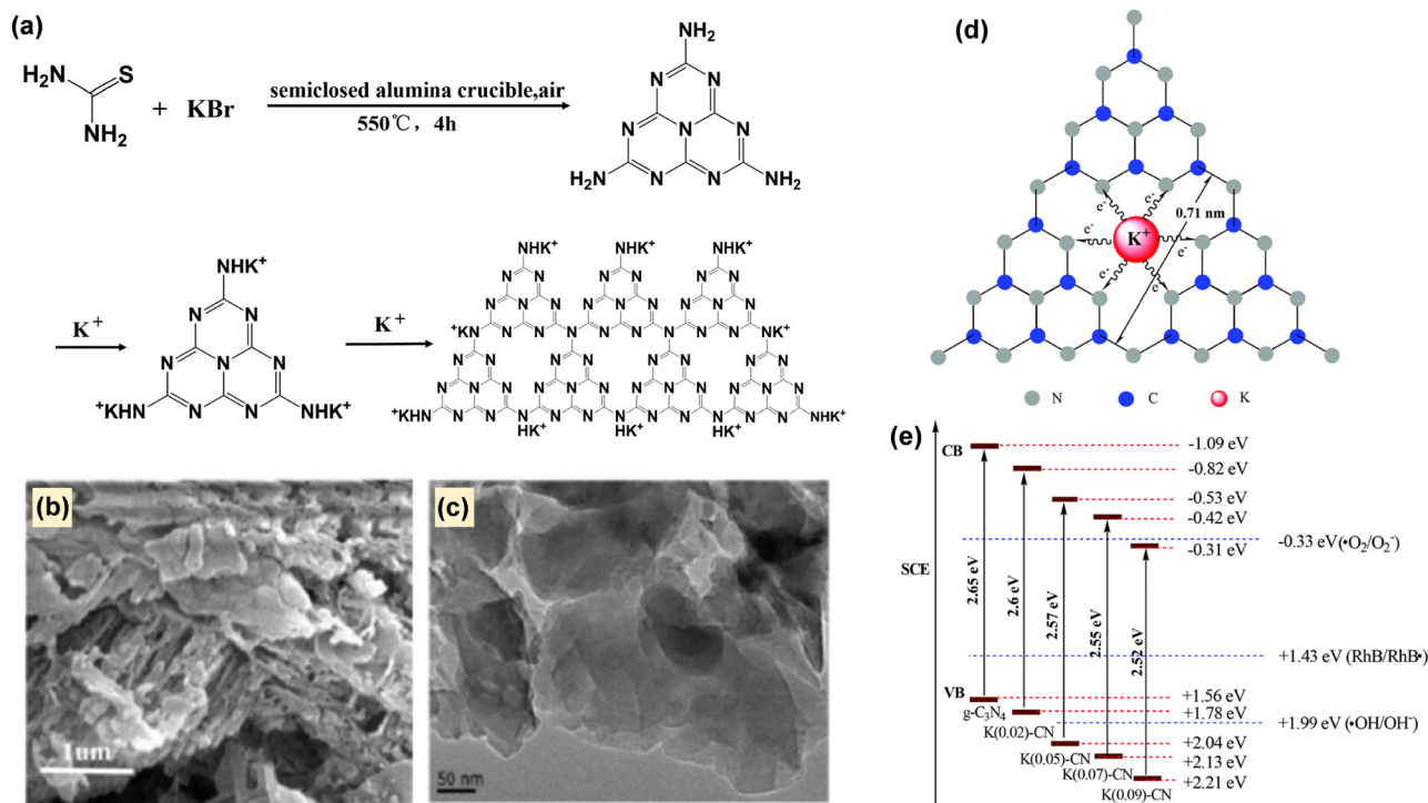
Fig. 13 (a) Schematic representation of the stepwise synthesis and (b) and (c) SEM and TEM pictures of K-CN-10. Reproduced with permission from ref. 88. Copyright 2018, Elsevier. (d) Illustration showing the possible doping sites of K^+ in K(x) -CN and (e) band structures of g - C_3N_4 and K(x) -CN (where x corresponds to the concentration of KOH, x = 0.02, 0.05, 0.07 , and 0.09 M). Reproduced with permission from ref. 90. Copyright 2015, Royal Society of Chemistry.
