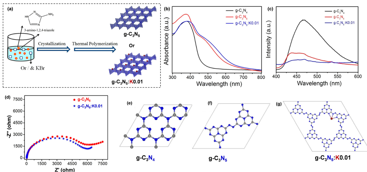
Fig. 23 (a) Schematic depiction of the synthesis of g\text{-C}_3\text{N}_5 and g\text{-C}_3\text{N}_5:\text{K}0.01 , (b) UV-vis DRS, (c) PL spectra, (d) EIS Nyquist plots of the synthesized samples, and (e)–(g) crystal structure models of g\text{-C}_3\text{N}_4 , g\text{-C}_3\text{N}_5 , and g\text{-C}_3\text{N}_5:\text{K}0.01 , respectively. Reproduced with permission from ref. 114. Copyright 2022, American Chemical Society.
