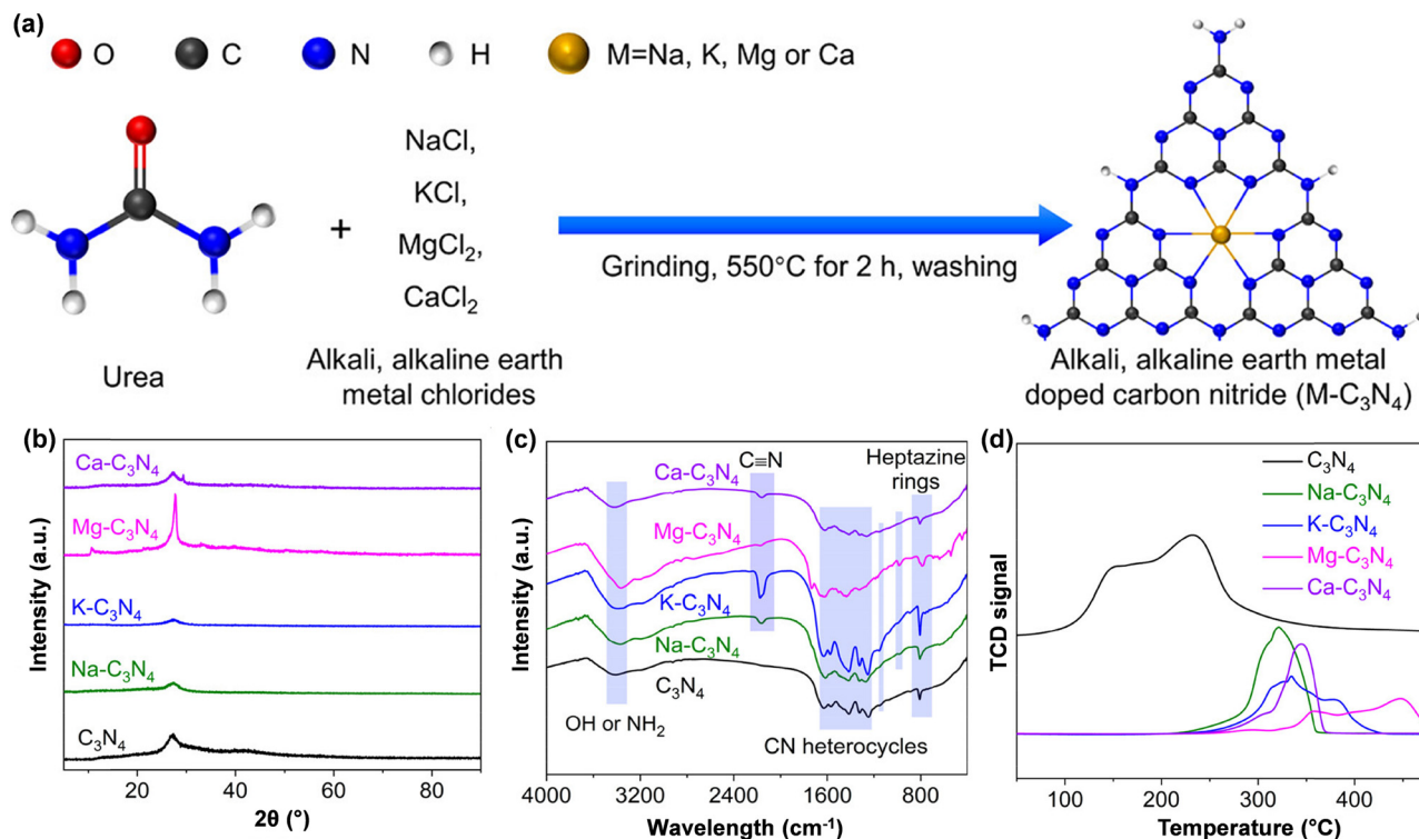
Fig. 34 (a) Diagrammatic illustration of the synthesis of M\text{-C}_3\text{N}_4 , (b) XRD patterns, (c) FT-IR spectra, and (d) \text{CO}_2 -TPD of all the prepared samples. Reproduced with permission from ref. 207. Copyright 2022, American Chemical Society.
