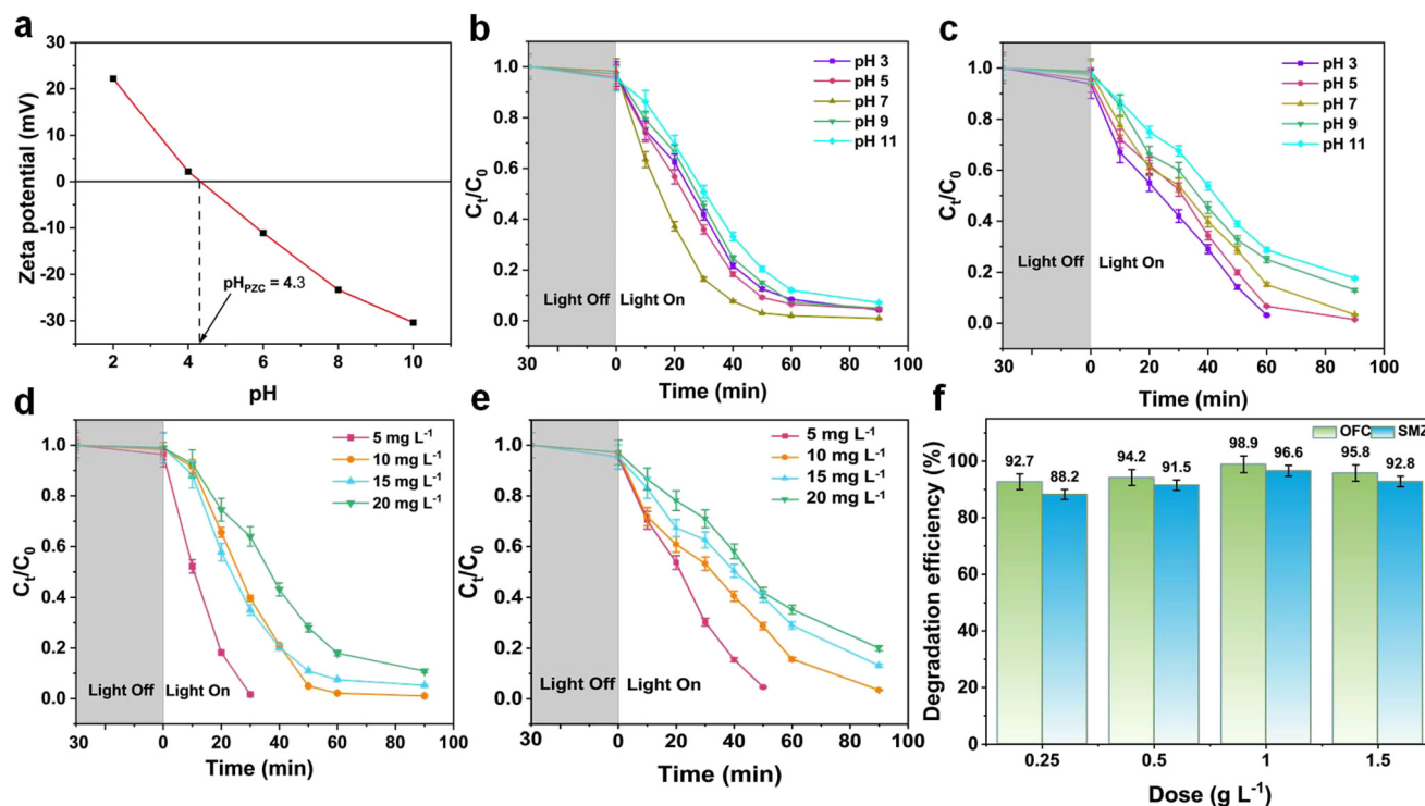
Fig. 7 (a) Zeta potential of F-GCN as a function of pH and point of zero charge (pHPzc). Effects of initial solution pH on the photocatalytic degradation of (b) OFC and (c) SMZ (experimental conditions: C_0 = 10 \text{ mg L}^{-1} ; photocatalyst dose = 1 \text{ g L}^{-1} ; temperature = 25 \text{ }^\circ\text{C} ). Effects of initial reactant concentration on the degradation of (d) OFC and (e) SMZ (experimental conditions: photocatalyst dose = 1 \text{ g L}^{-1} ; temperature = 25 \text{ }^\circ\text{C} ). (f) Effects of photocatalyst dosage on the degradation of OFC and SMZ (experimental conditions: C_0 = 10 \text{ mg L}^{-1} ; temperature = 25 \text{ }^\circ\text{C} ).
