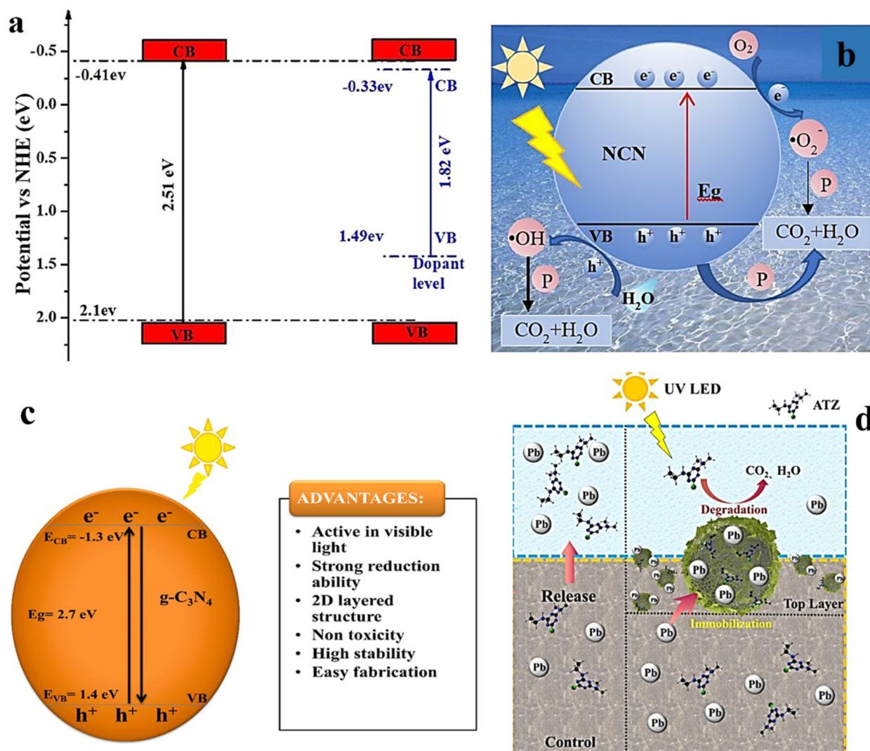
Fig. 10 (a and b) Charge separation mechanism and transport of photogenerated electron-hole pairs at N-doped g-C_3N_4 , respectively. Reproduced with permission from ref. 208 (adapted from ref. 208 with permission from Elsevier, Copyright 2021). (c) Advantages of g-C_3N_4 in photocatalysis. Reproduced with permission from ref. 209 (adapted from ref. 209 with permission from Elsevier, CC-BY-NY licence). (d) Decontamination of ATZ and Pb in paddy soil using alkalised biochar and g-C_3N_4 composite 234 (adapted from ref. 234 with permission from Elsevier, Copyright 2023).
