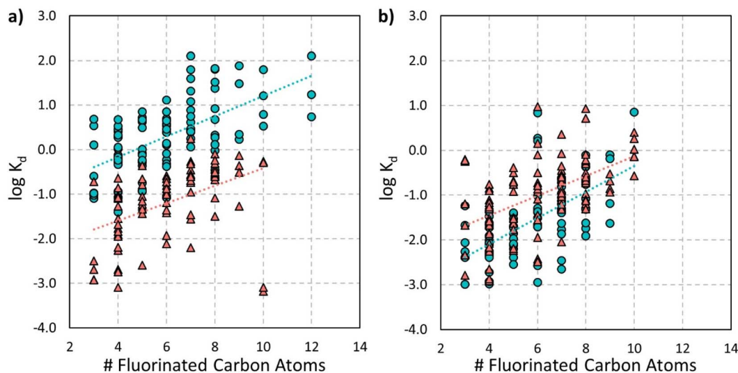
Fig. 5 Relationship between average \log K_d values (units are L\ g^{-1} prior to log transformation) and the number of fluorinated carbon atoms in each PFAS for (a) the iron oxide minerals ferrhydrite (blue circles) and goethite (red triangles) and (b) silica clay minerals kaolinite (blue circles) and montmorillonite (red triangles). Zwitterions are not included in this plot because they all have five or six fluorinated carbon atoms, yielding insufficient data to observe a relationship.
