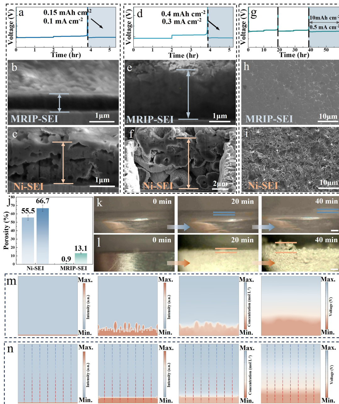
Fig. 5 Deposition behaviors on various current collectors. (a) Charge/discharge profiles and corresponding FIB-SEM images with (b) the MRIP-SEI and (c) the Ni-SEI at 0.1\text{ mA cm}^{-2} . (d) Charge/discharge profiles and corresponding FIB-SEM images with (e) the MRIP-SEI and (f) the Ni-SEI at 0.3\text{ mA cm}^{-2} . (g) Charge/discharge profiles and corresponding SEM images with (h) the MRIP-SEI and (i) the Ni-SEI at 0.5\text{ mA cm}^{-2} . (j) Comparison of porosity of lithium deposition layers induced by different current collectors. Morphological evolution of electrodeposited Li characterized by real-time optical microscopy with (k) the MRIP-SEI and (l) the Ni-SEI. Phase field simulation results of lithium deposition induced by (m) heterogeneous nucleation (Ni-SEI) and (n) uniform nucleation (MRIP-SEI).
