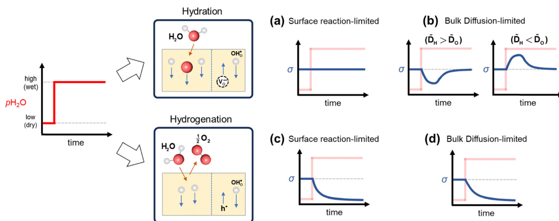
Fig. 2 Schematic illustration of surface reaction and charge transport processes and corresponding electrical conductivity relaxation (ECR) behaviors for hydration-type (a and b) and hydrogenation type (c and d) proton uptake mechanisms. Each panel shows typical relaxation behavior under surface reaction-limited (a and c) and bulk diffusion-limited (b and d) cases.
