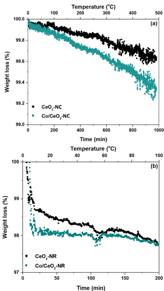
Fig. 8 Thermogravimetric curves of (a) \text{CeO}_2\text{-NC} and \text{Co/CeO}_2\text{-NC} , (b) \text{CeO}_2\text{-NR} and \text{Co/CeO}_2\text{-NR} .
