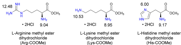
Fig. 1 Amino acid precursors used in the synthesis of the catalyst. The \text{pK}_a values for the amino acid form of these compounds are shown next to each basic group. 41
